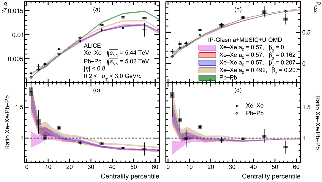
Fig. 4. Panels (a) and (b): Charged particle v_{4,22} (left) and \rho_{4,22} (right) as a function of centrality in Xe-Xe and Pb-Pb collisions at \sqrt{s_{NN}} = 5.44 TeV and \sqrt{s_{NN}} = 5.02 TeV, respectively. Panels (c) and (d): Ratio between Xe-Xe and Pb-Pb v_{4,22} (left) and \rho_{4,22} (right). Statistical and systematical uncertainties are shown as vertical lines and grey boxes, respectively. The measurements are compared with IP-Glasma + MUSIC + UrQMD calculations [99,100] to constrain the \beta_2 and a_0 parameters of ^{129}\text{Xe} nuclei. The thickness of the bands represent statistical uncertainties.
