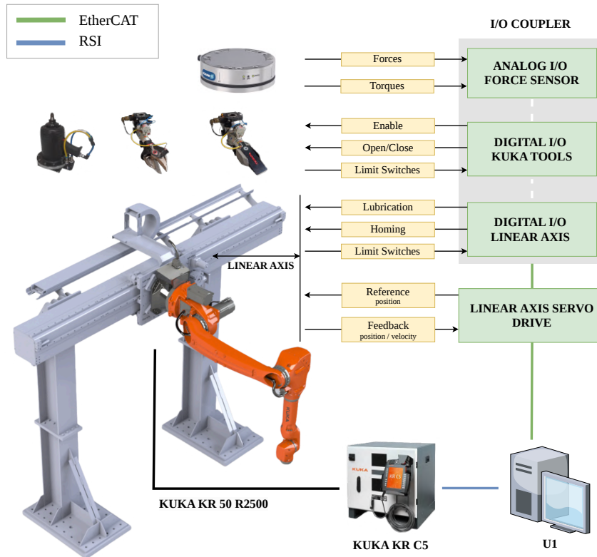
Figure 5. EtherCAT and RSI (Robot Sensor Interface) connection diagram within the R1 subsystem. Green lines represent EtherCAT-based communications, and blue lines indicate RSI connections.
