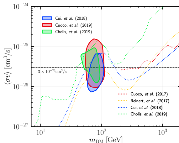
Figure 5. The regions of DM parameter space favored by recent analyses of AMS-02 antiproton data for the case of annihilations into b\bar{b} , in the plane of velocity averaged annihilation cross section \langle\sigma v\rangle and DM mass m_{\text{DM}} . The contours of Cuoco, et al. 2019 [28] (red) and Cholis, et al. 2019 [29] (green) refer to the 2\sigma best-fit region in the frequentist interpretation, while the contour of Cui, et al. 2018 [70] (blue) corresponds to a 95% C.L. in Bayesian interpretation. The exclusion limits from four recent analysis are also shown [27, 29, 70, 72]. We note that the analysis of Reinert, et al. 2017 [27] does not find a significant DM signal, but the derived limit weakens at m_{\text{DM}} \approx 80 GeV such that all indicated DM signal regions lie partly below this limit. For a thermal WIMP one would expect a annihilation cross section at the order of \langle\sigma v\rangle \approx 3 \times 10^{-26} \text{ cm}^3/\text{s} (black dashed line). The signal regions and limits have been rescaled to a local DM density of \rho_0 = 0.3 \text{ GeV}/\text{cm}^3 . Note that the different analyses use slightly different values for the halo half-height which affects the value of \langle\sigma v\rangle .
