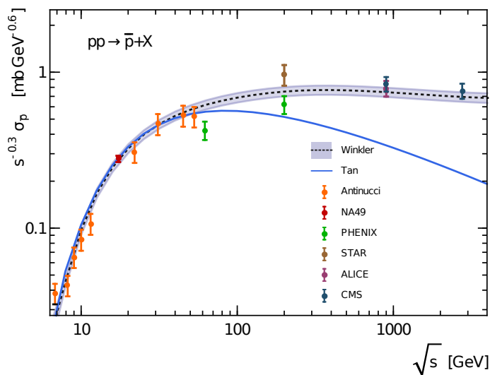
Figure 9. Antiproton production cross section in proton-proton interactions [24].
