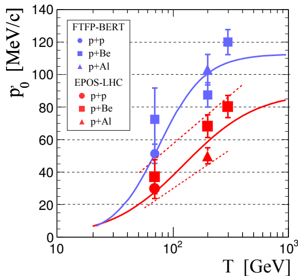
Figure 10. p'_0 for antideuterons as function of kinetic energy of the incoming proton for two different hadronic generators. The solid lines show empiric fits to the best-fit p'_0 values for the corresponding generator. The dashed red lines indicate the one-sigma uncertainty range for EPOS-LHC [121].
