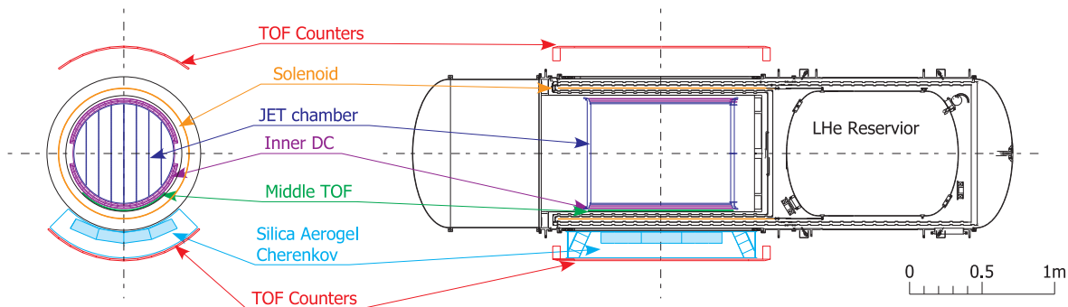
Figure 1. The BESS-Polar II experiment consists of inner drift chambers and a jet-type drift tracking chamber, surrounded by a solenoid magnet, aerogel Cherenkov counter, and time-of-flight system. Reprinted with permission from [53].
