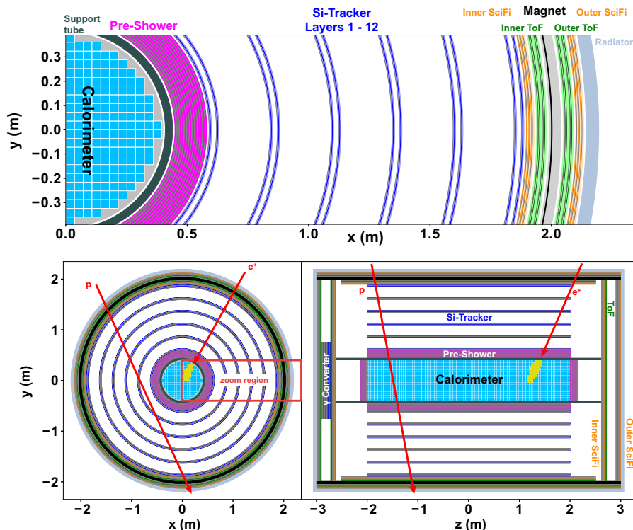
Figure 14. The AMS-100 instrument consists of a central calorimeter surrounded by a silicon-strip and scintillating-fiber tracker, all within a high-temperature superconducting solenoid magnet. Figure from [204].
