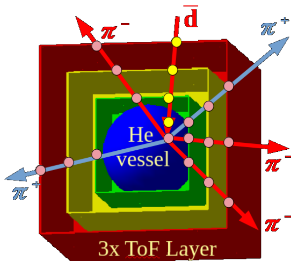
Figure 13. The ADHD instrument is made of a 400 bar helium-gas calorimeter (HeCal) surrounded by a time-of-flight system with three scintillator layers. Antideuterons are detected as a single in-going prompt track (yellow points) followed by several out-going delayed pions (light-red points).
