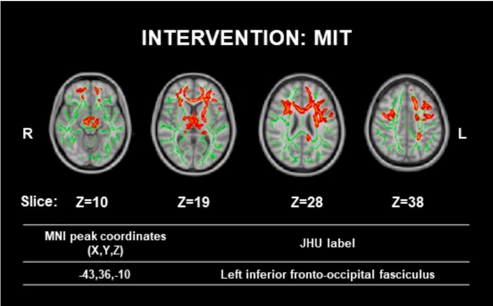
Fig. 1. Effect of Metacognitive Interpersonal Therapy (MIT) on fractional anisotropy (FA). Red-to-yellow voxels denote areas of increased FA after MIT intervention ( p < .05 , TFCE and FWER corrected). Voxels were thickened using tbss_fill , to aid visualization. No significant difference was observed after standard clinical management intervention. The standard Johns Hopkins University (JHU) white-matter tractography atlas was overlaid to the statistical map in order to identify the anatomical location of local maxima peak of significant clusters. (For interpretation of the references to color in this figure legend, the reader is referred to the web version of this article.)
