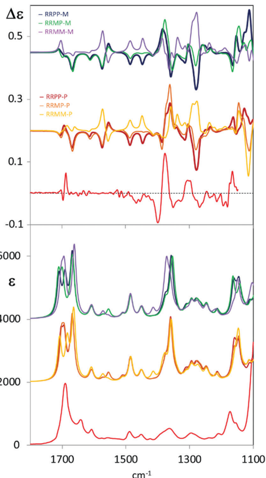
Fig. 3 Comparison of experimental VCD spectra of C_6F@R,R-1 (top) and IR absorption spectra of C_6F@R,R-1 with calculated VCD and IR spectra of C_6F@R,R-1 with the two head groups and fluorinated chains in all possible configurations ( PP-M , PP-P , MM-M , MM-P , MP-M , MP-P ). Experimental data in red.
