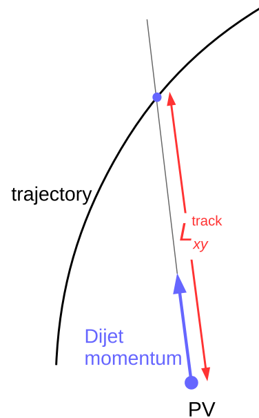
FIG. 1 (color online). Diagram showing the calculation of the distance L_{xy}^{\text{track}} . In the transverse plane, L_{xy}^{\text{track}} is the distance along the dijet momentum vector from the primary vertex (PV) to the point at which the track trajectory is crossed.
