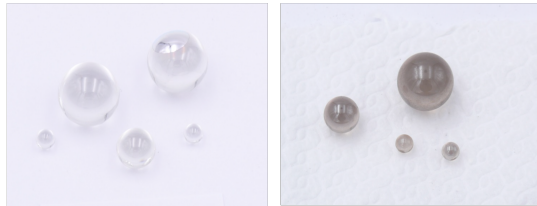
Fig. 2. Precision components for alignment systems: glass balls unirradiated (left) and irradiated at 10 MGy of gamma dose (right). Acknowledgement: M. Sosin.
