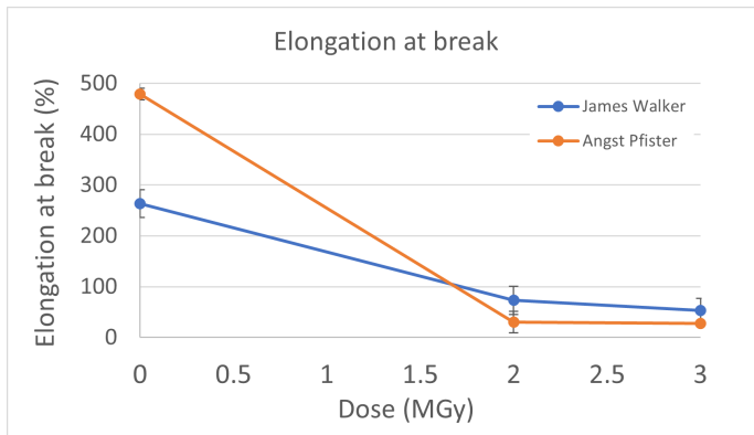
Fig. 5. Elongation at break of James Walker Shieldseal 663@ (blue) and of Angst+Pfister EPDM 70.20-10 (orange) as a function of the gamma dose. The line connecting the points is a guide for the eyes only.
