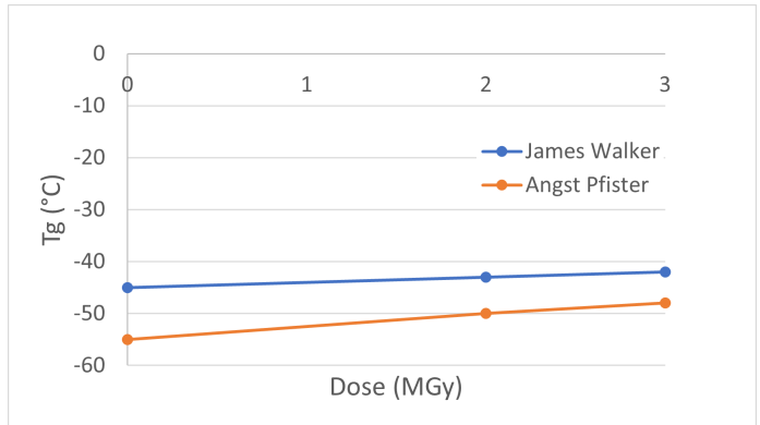
Fig. 6. Glass transition temperature T_g of James Walker Shieldseal 663@ (blue) and of Angst+Pfister EPDM 70.20-10 (orange) as a function of the gamma dose. The line connecting the points is a guide for the eyes only.
