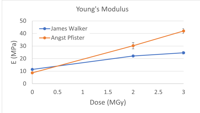
Fig. 4. Young's Modulus E of James Walker Shieldseal 663@ (blue) and of Angst+Pfister EPDM 70.20-10 (orange) as a function of the gamma dose. The line connecting the points is a guide for the eyes only.
