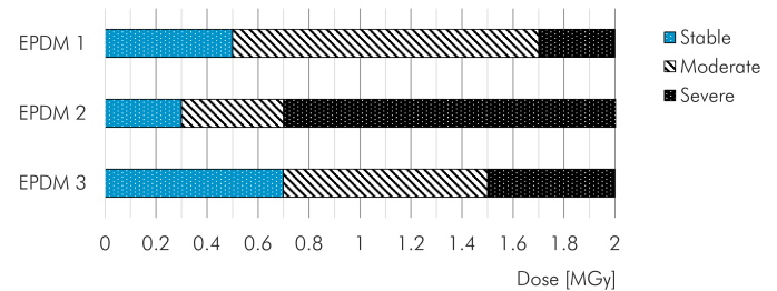
Fig. 8. Dose thresholds for three commercial EPDM O-rings irradiated in mixed neutron and gamma radiation. In the graph, EPDM 3 corresponds to James Walker Shieldseal663®. Data extracted and elaborated from [17], [18].
