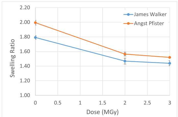
Fig. 7. Swelling ratio SR_{eq} of James Walker Shieldseal 663@ (blue) and of Angst+Pfister EPDM 70.20-10 (orange) as a function of the gamma dose. The line connecting the points is a guide for the eyes only.
