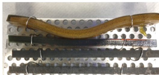
Fig. 1. Four materials candidate for the protective covers of magnets after gamma irradiation at 10 MGy. Acknowledgement: C. L. Marraco Borderas.
