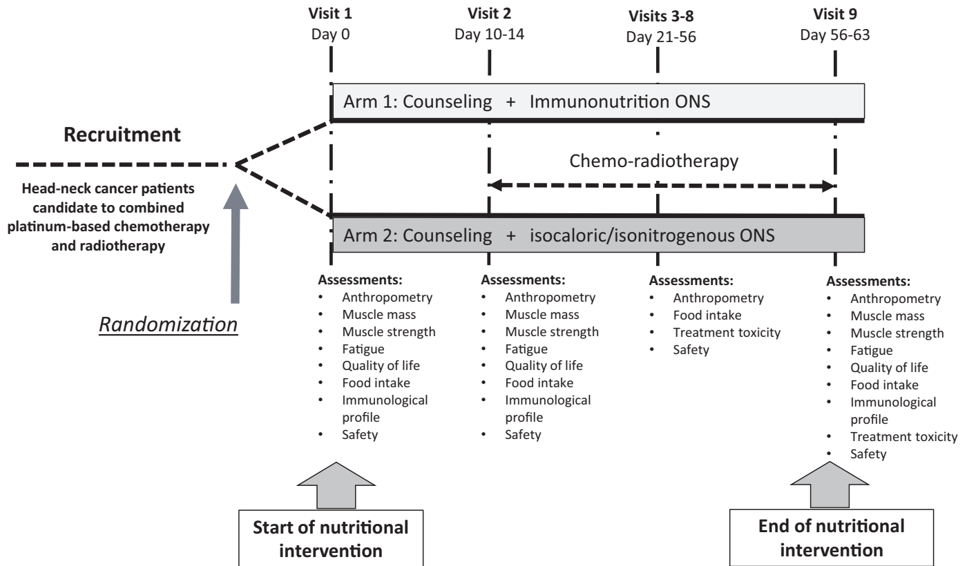
Figure 1. Study flowchart.
