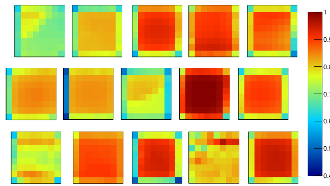
Figure 86. Map of the relative quantum efficiency (QE) of the MCP-PMTs used during the prototype test at CERN in 2015, as implemented in simulations. The absolute values of the QE the MCP-PMTs are determined as the product of this map with the wavelength-dependent QE from figure 87.
