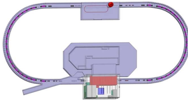
Figure 2. The HESR ring with the \bar{P} ANDA experimental area at the bottom and the electron cooler installation at the top. Standard operation has the antiproton injection from RESR (during the modularized startup phase from CR) from the left, or protons at reversed field polarities. Reproduced from http://inspirehep.net/record/1189529/export/hx . CC BY 3.0.
