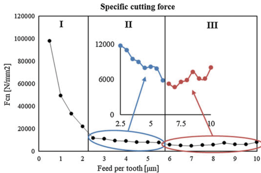
Fig. 5 Specific cutting forces versus feed per tooth
