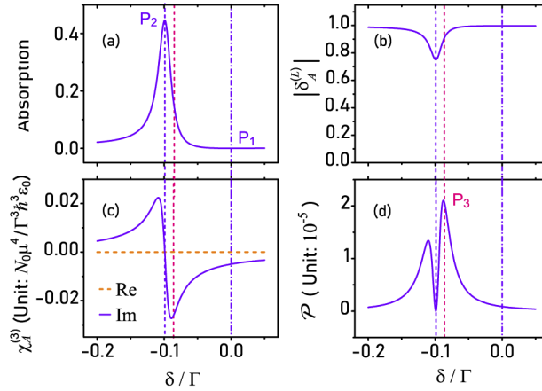
Fig. 2. Large Detuning Color-Entanglement Generation. (a) Absorption \mathcal{R} , (b) modulus of the mismatch function \delta_A^{(L)} , (c) real and imaginary part of the nonlinear susceptibility \chi_A^{(3)} and (d) generation efficiency \mathcal{P} as a function of the Stokes ( \omega_s ) two-photon detuning \delta (Panel A Fig. 1). Here \Delta_c = \Delta_{c'} = 10 \Gamma , \Delta_d = -10 \Gamma , \Omega_c = \Omega_{c'} = 0.5 \Gamma , \Omega_d = \sqrt{2}\Omega_c . Plots in each panel are the same for Stokes photon \omega_{s'} (Panel B Fig. 1). Characteristics points in the Stokes generation process are marked by vertical lines representing maximum generation efficiency ( P_3 ), maximum ( P_2 ) and minimum ( P_1 ) absorption. Optimal efficiency occurs for Stokes photons at wavelengths \lambda_s = 795.522 \text{ nm} , \lambda'_s = 795.521 \text{ nm} , with equal detuning ( \delta = -0.08\Gamma ) from the relevant transitions, whereas the anti-Stokes photon is emitted at \lambda_{as} = 780.778 \text{ nm} . The sample is L = 100 \mu\text{m} long and contains atoms with an average density of N_0 = 5 \times 10^{11} \text{ cm}^{-3} while other atomic parameters are as in Fig. 1.
