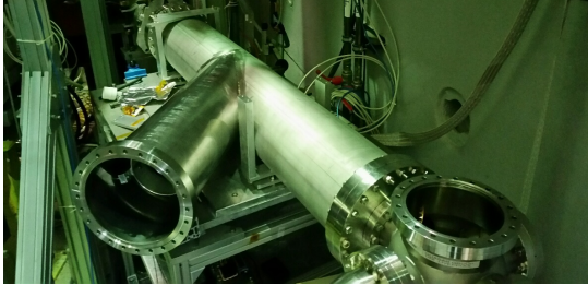
Figure 3. The GRACE beamline at the end of one of the extraction points of the AD before the detector chamber is mounted. The detector chamber is installed on the open flange on the left.
