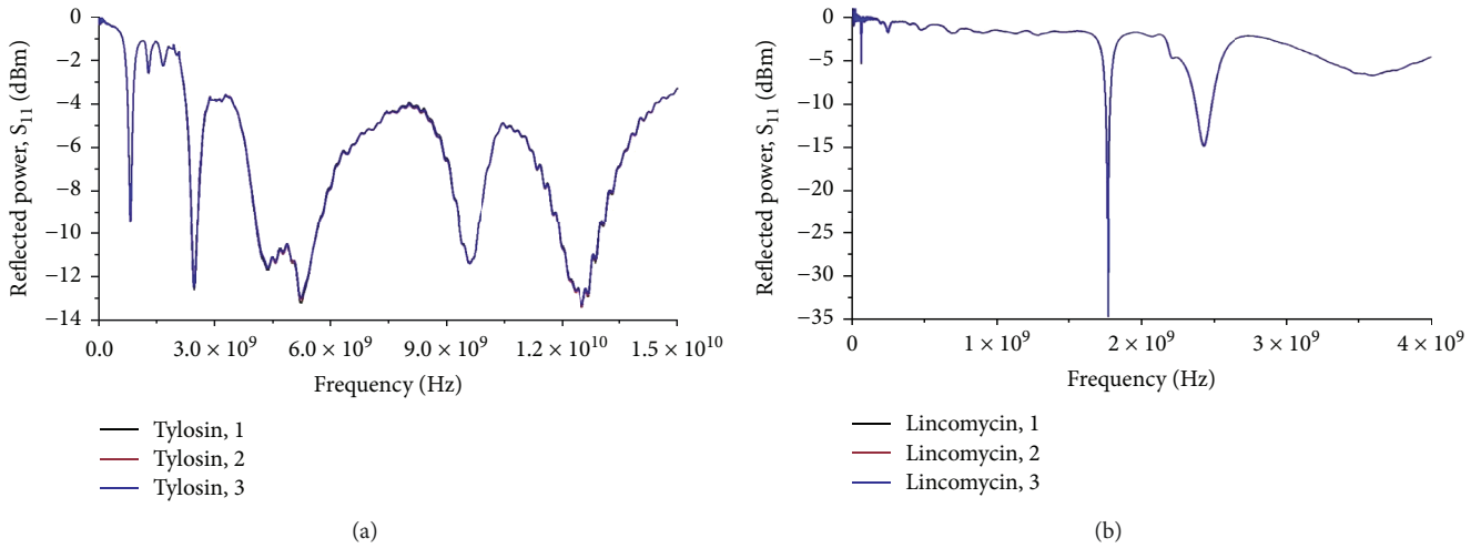
FIGURE 10: (a) Repeatability of tylosin's sample at the lowest concentration of 0.20 \mu\text{g/l} with IDE sensor using the full-range frequencies: 0 \text{ Hz} - 1.5 \times 10^{10} \text{ Hz} ; (b) repeatability of lincomycin sample at the lowest concentration of 0.25 \mu\text{g/l} with hairpin resonator sensor using the full-range frequencies: 0 \text{ Hz} - 4 \times 10^9 \text{ Hz} .
