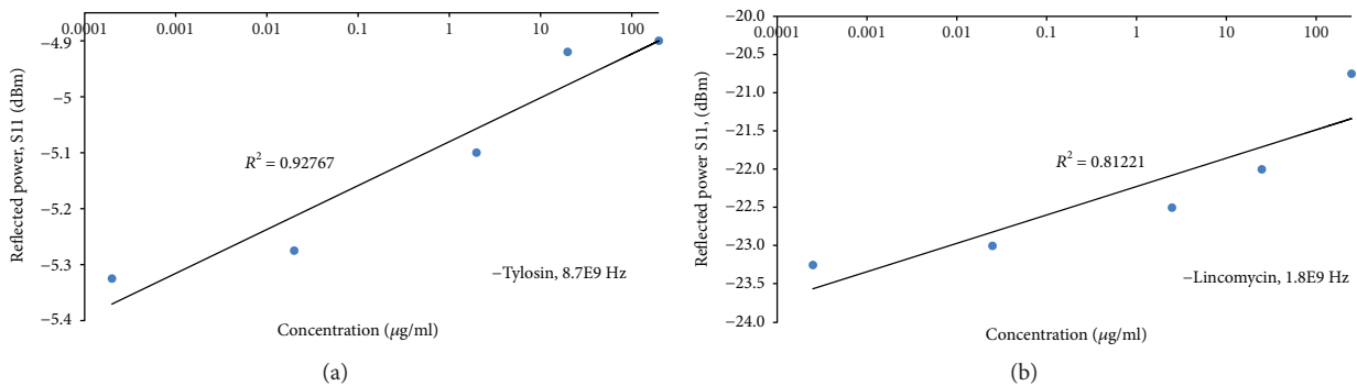
FIGURE 12: (a) Dependence of the S_{11} transmitted microwave signal on tylosin concentration at 8.7 \times 10^9 \text{ Hz} recorded for 400 \mu\text{l} solution placed in IDE sensor; (b) dependence of the S_{11} transmitted microwave signal on lincomycin concentration at 1.8 \times 10^9 \text{ Hz} recorded for 200 \mu\text{l} solution placed in hairpin resonator sensor.
