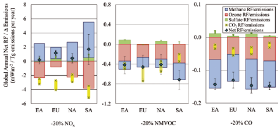
Figure 5.5 Radiative forcing from NO x , VOC and CO emissions. (from Fry et al. 2012).
