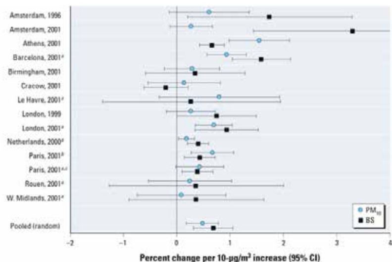
Figure 2.3 Single-city estimates of all-cause mortality for PM 10 and black smoke BS (10 mg m -3 of BS correspond about to 1 mg m -3 of BC). Year indicates year of publication (Janssen et al. 2011 and reference therein)
