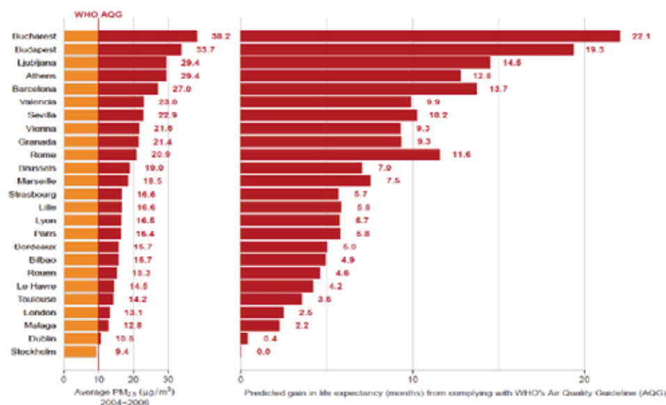
Figure 1.3 Predicted average gain in life expectancy (months) at age 30 in 25 Apekom cities for a decrease in average annual level of PM 2.5 to 10µg/m 3 (WHO's Air Quality Guideline). Source: www.APHEKOM.org
