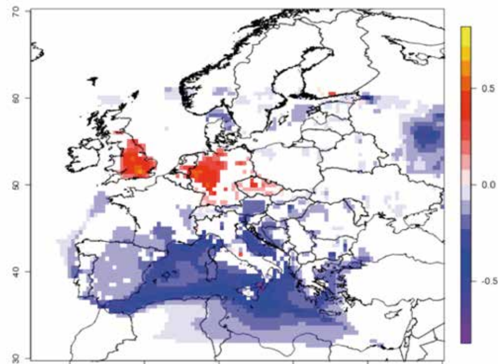
Figure 3.5 Ensemble model mean trend of ozone owing to the change in anthropogenic emission evolution alone (Colette et al. 2011).
