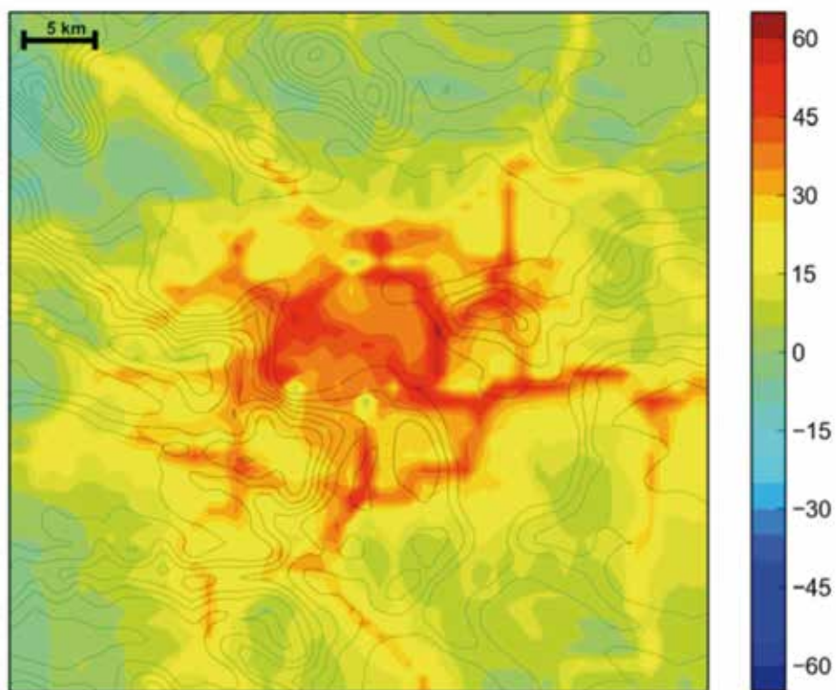
Figure 3.4 Difference map for \text{O}_3 concentrations (units are \text{mg m}^{-3} ) in the Paris metropolitan area, calculated with baseline and the zeroed out traffic emissions (from MEGAPOLI Pandis et al. 2010).
