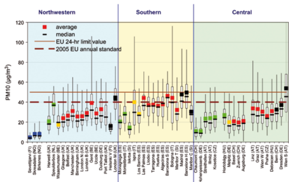
Figure 2.4 Annual average PM10 concentration in different geographical areas in Europe (Northwestern, Southern, Central) in remote (blue), rural (green), near city (yellow), urban background (red), and kerbside (black) sites (Putaud et al. 2010).
