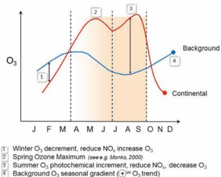
Figure 3.1 A schematic diagram of an idealized marine background and European continental ozone seasonal cycle (Wilson et al. 2012)
