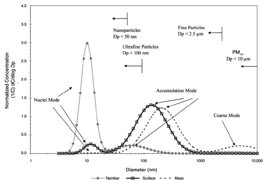
Figure 2.1 Normalized size distribution of particle number, surface, and mass for a typical roadside PM (HEI 2010).
