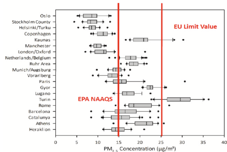
Figure 1.1 Annual mean PM 2.5 concentrations measured in the ESCAPE project (Eeftens et al. 2012a).
