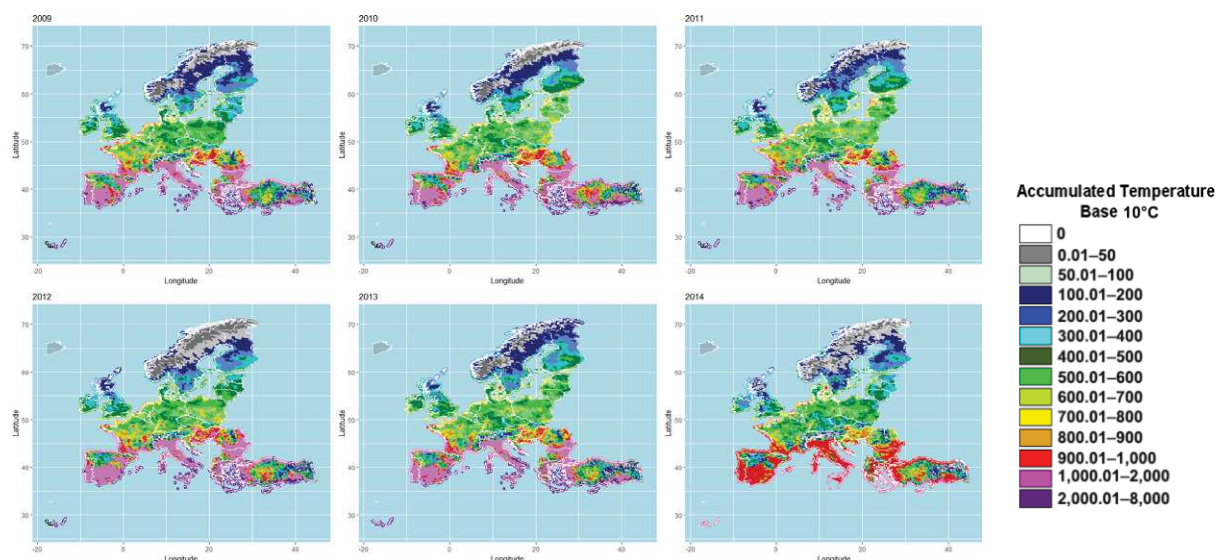
Figure E.3: Accumulated temperature in Europe above 10°C for years 2009–2014
