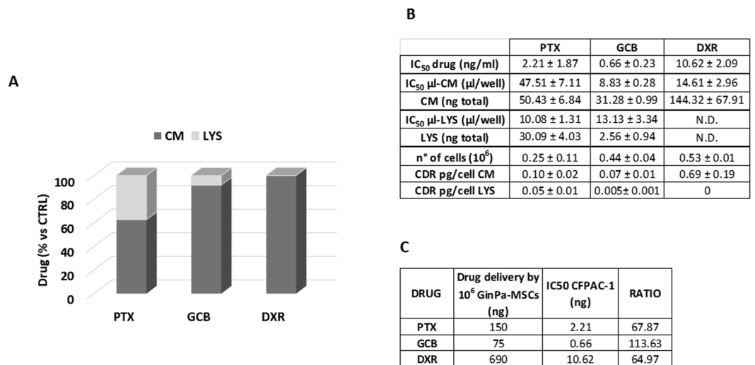
Figure 4. Percentage of drug incorporated and released. The histogram (A) reports the percentage of drugs estimated by biological dosage in the conditioned medium (CM) and cell lysate (LYS). The box (B) reports the IC 50 value of the drugs (ng/ml) of the conditioned medium and lysate (μl/well) used to estimate the amount of drugs incorporated (LYS, ng total) or released (CM, ng total) by GinPa-MSCs. Values are expressed as mean ± standard deviation (SD) of three independent experiments. The box (C) reports the amount of drugs potentially delivered by 10 6 GinPa-MSCs and their ratio to the IC 50 values of each drug. CDR = Single cell drug release.
