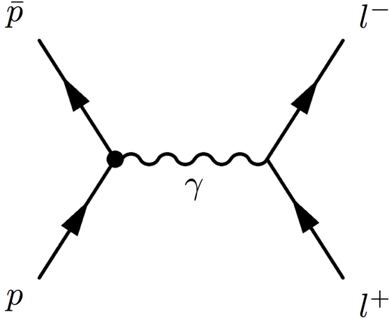
Figure 1: Tree-level contributing diagram to \bar{p}p \rightarrow l^+l^- .
