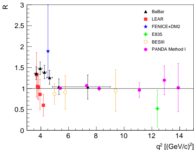
Figure 15: Form factor ratio extracted from the present simulation (magenta circles) as a function of q^2 , compared with the existing data. Data are from Ref. [12] (red squares), Ref. [13] (black triangles), Ref. [72] (open orange circles), and Ref. [73] (green cross and blue star).
