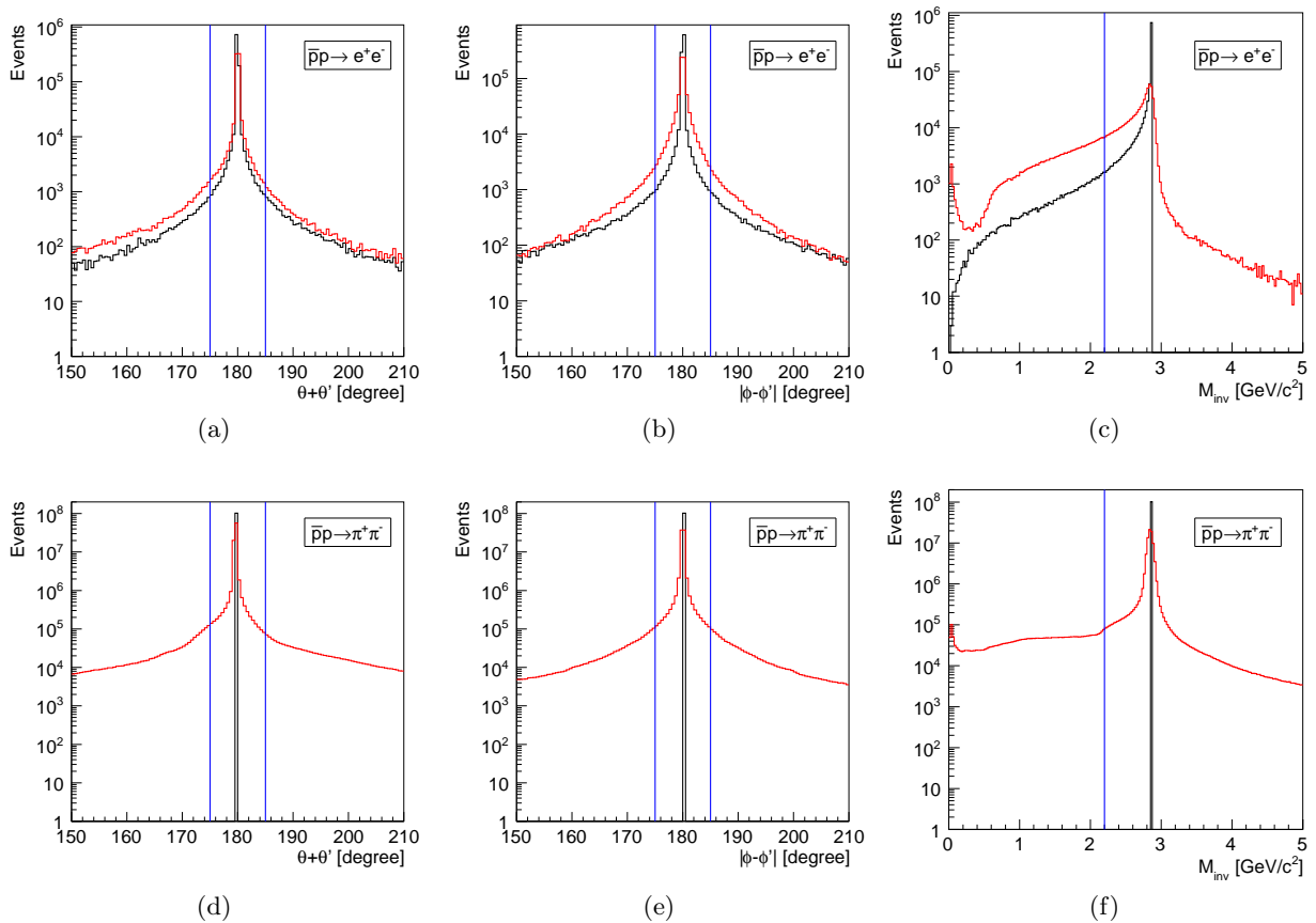
Figure 11: Spectra of generated (black) and reconstructed (red) events for different kinematic variables for the signal (top row) and the background (bottom row) at p_{lab} = 3.3 \text{ GeV}/c : (a, d) the sum of the polar angles in the c.m. frame; (b, e) the difference in the azimuthal angles in the c.m. frame; (c, f) the invariant mass of the reconstructed particles. The blue lines denote the range of the variable accepted for further analysis.
