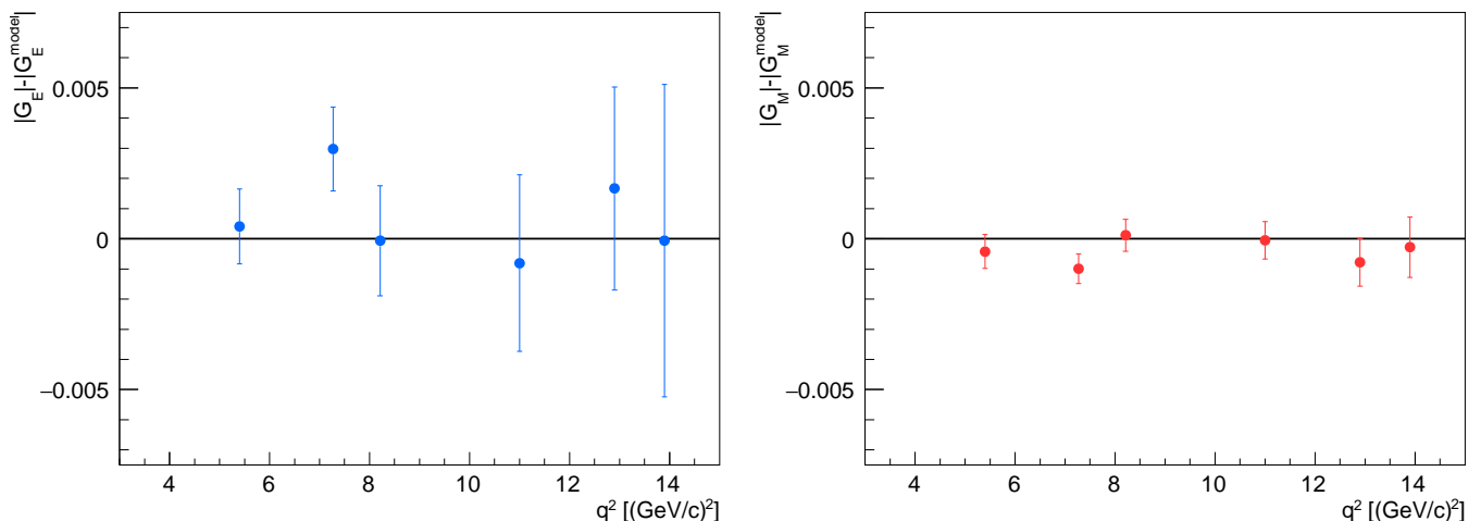
Figure 16: Residual values of |G_E| (left panel) and |G_M| (right panel) for different q^2 values with statistical uncertainties only (Method I).
