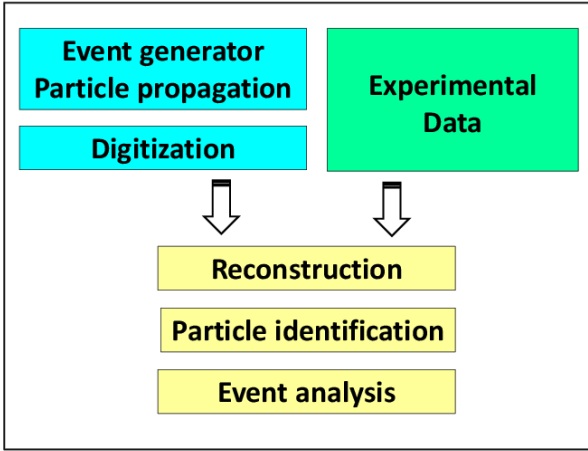
Figure 6: Standard analysis chain in PandaRoot.
