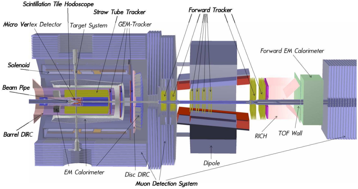
Figure 5: View of the \bar{P} ANDA detector.
