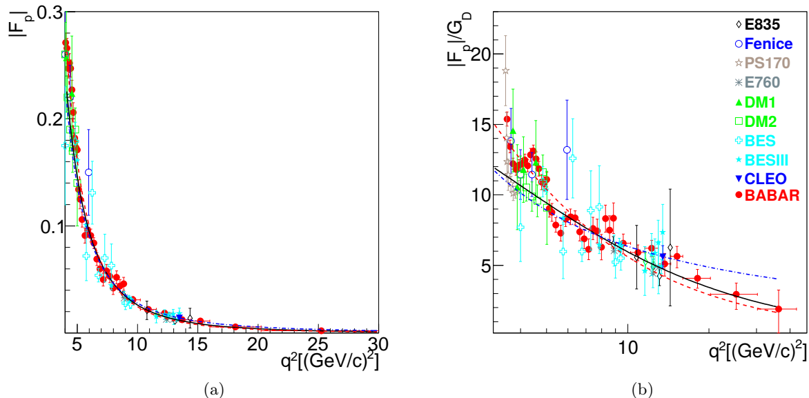
Figure 2: q^2 dependence of the world data for \bar{p}p \rightarrow e^+e^- and e^+e^- \rightarrow \bar{p}p . The effective proton TL FF, |F_P| , is extracted from the annihilation cross sections assuming |G_E| = |G_M| : E835 [35, 36], Fenice [37], PS170 [12], E760 [38], DM1 [39], DM2 [40, 41], BES [42], BESIII [14], CLEO [43], BABAR [32, 33]. Different parameterizations are shown based on Eq. (11) (solid black and dashed red lines) and from Eq. (10) (dash-dotted blue line), as described in the text.
