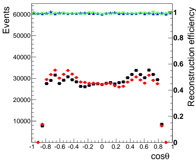
Figure 17: Angular distribution in the c.m. system of the Monte Carlo events for e^- (green asterisks) and e^+ (blue triangles) generated according to the PHSP, for p_{lab} = 3.3 GeV/c. The reconstructed events after the cuts are also shown for e^- (black squares) and e^+ (red circles). The right y -axis represents the efficiency values.
