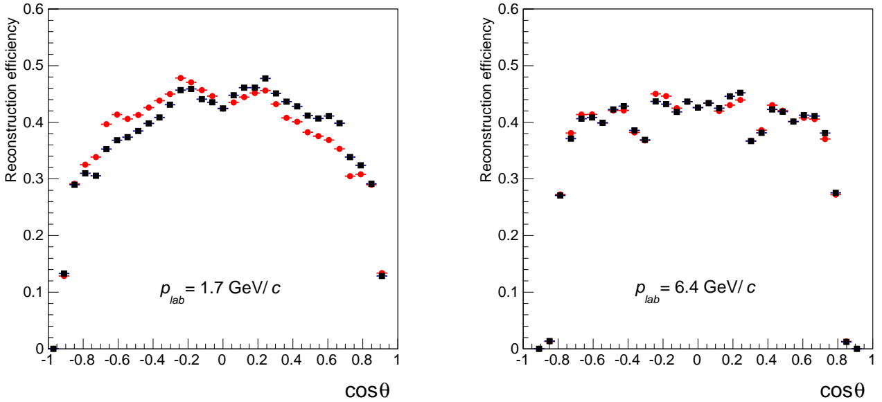
Figure 18: Signal efficiency for e^+ (red circles) and e^- (black squares) as a function of \cos\theta in the c.m. system: (left panel) p_{lab} = 1.7 and (right panel) 6.4 GeV/ c .
