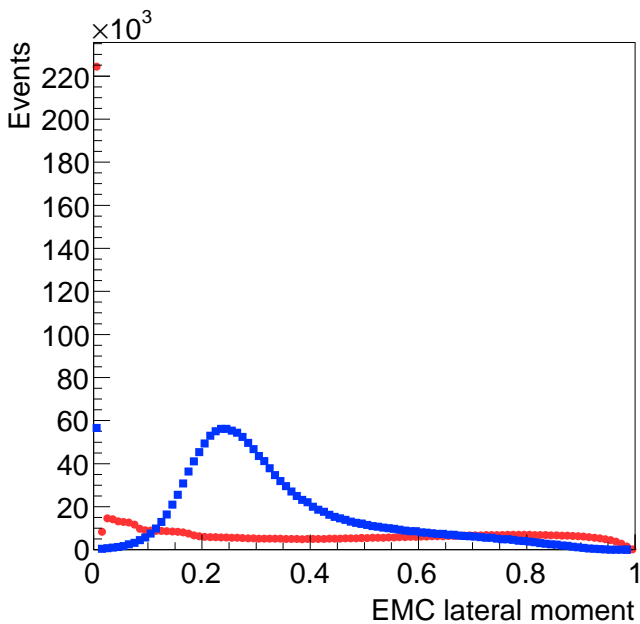
Figure 8: EMC lateral moment for the signal (blue squares) and background (red circles) events for p_{lab} = 3.3 GeV/c.
