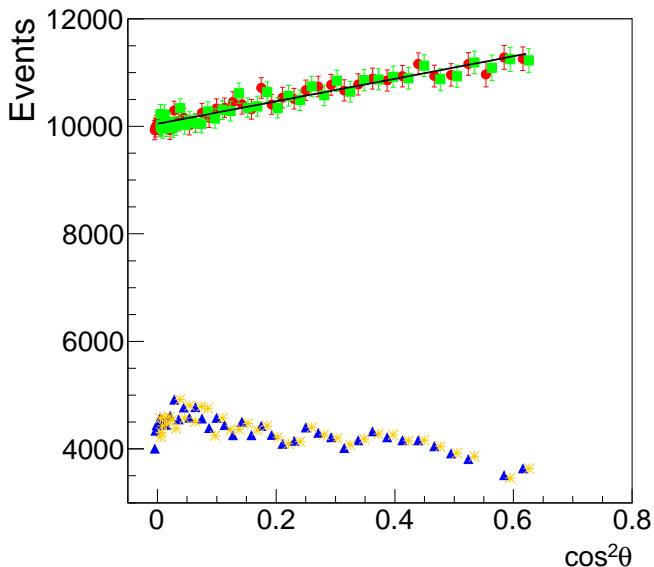
Figure 19: Observed number of events before efficiency correction O(\cos\theta) (forward events (blue triangles) and backward events (orange stars)) and after efficiency correction F(\cos\theta) (forward events (red circles) and backward events (green squares)), as a function of \cos^2\theta for p_{lab} = 1.7 GeV/c, assuming R = 1 . The solid black line represents the linear fit. The abscissa for backward (forward) events is shifted by +0.005 ( -0.005 ) for better visualization.
