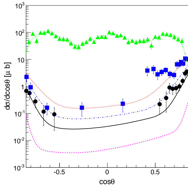
Figure 3: Data and modeling of the \pi^- angular distributions from the reaction \bar{p}p \rightarrow \pi^+\pi^- , as a function of \cos\theta , for different values of the beam momentum: p_{lab} = 1.7 \text{ GeV}/c [22] (green triangles and dash-triple dotted line); p_{lab} = 5 \text{ GeV}/c [49] (blue full squares and dash-dotted line); p_{lab} = 6.21 \text{ GeV}/c [50] (black full circles and solid line). The results of the generator [46] are also given at p_{lab} = 3 \text{ GeV}/c (red dotted line) and p_{lab} = 10 \text{ GeV}/c (magenta dashed line).
