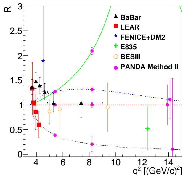
Figure 20: Expected statistic precision on the determination of the proton FF ratio from the present simulation (magenta circles) as a function of q^2 , compared with the existing data. Data are from Ref. [12] (red squares), Ref. [13] (black triangles), Ref. [72] (open orange circles), and Ref. [73] (green cross and blue stars). The statistical uncertainties are extracted in the angular range |\cos\theta| \leq 0.8 . Curves are the graphic representations related to the theoretical predictions, as explained in the text.
