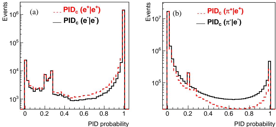
Figure 10: (a) Total PID probability distribution for a e^+ to be identified as a e^+ \text{PID}_c(e^+|e^+) (dashed red line) and for an e^- to be identified as an e^- \text{PID}_c(e^-|e^-) (solid black line). (b) Total PID probability distribution for a \pi^+ to be identified as a e^+ \text{PID}_c(\pi^+|e^+) (dashed red line) and for a \pi^- to be identified as an e^- \text{PID}_c(\pi^-|e^-) (solid black line). p_{lab} = 3.3 \text{ GeV}/c .
