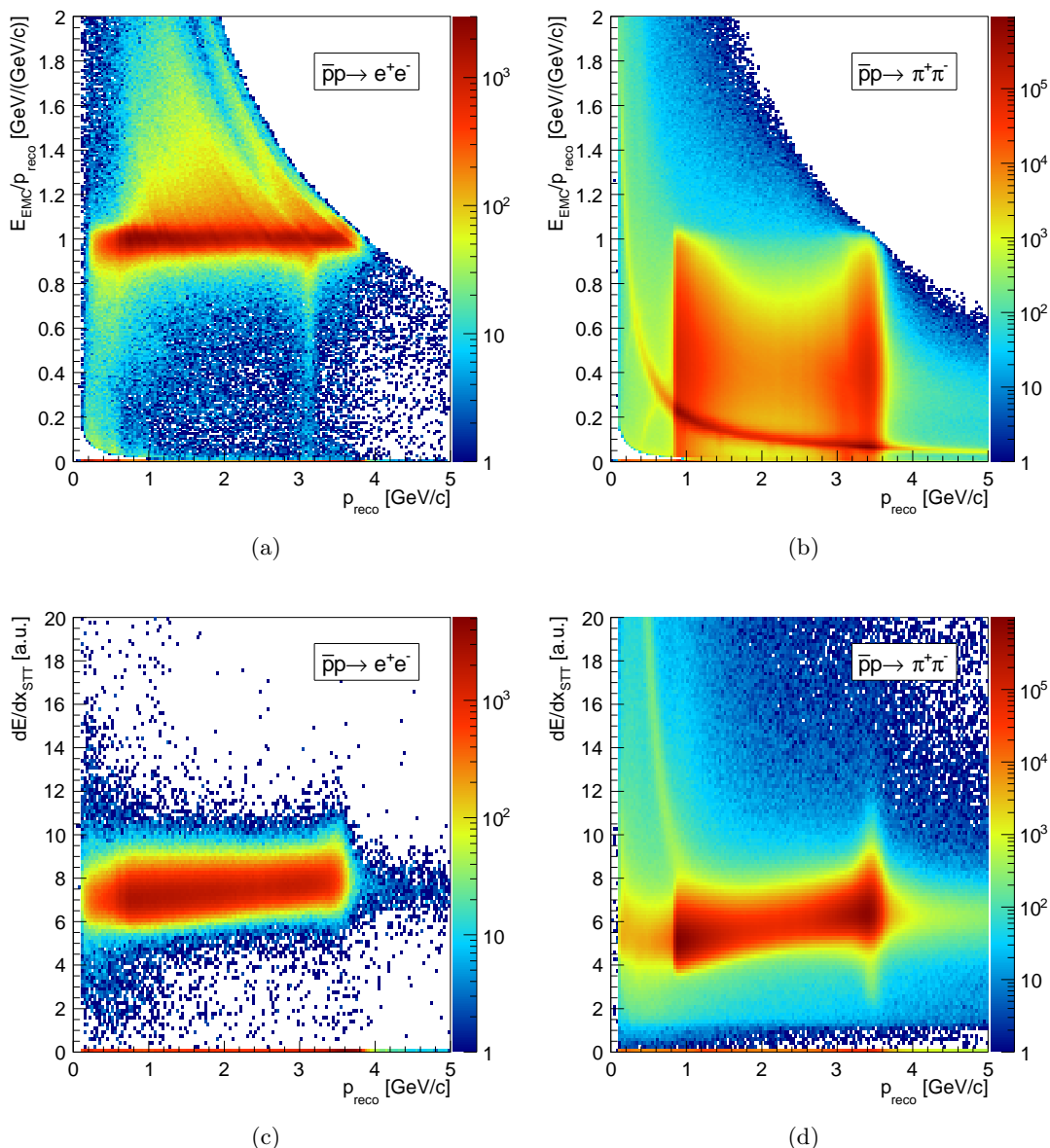
Figure 9: Detector response to the signal (left column) and the background (right column): (a,b) is the ratio of the energy deposited in the EMC to the reconstructed momentum; (c,d) is the energy loss per unit of length in the STT as a function of momentum at p_{\text{lab}} = 3.3 GeV/c.
