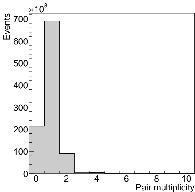
Figure 12: Multiplicity distribution of the number of reconstructed pairs of particles. 10^6 signal events were generated at a beam momentum of p_{lab} = 3.3 GeV/c.
