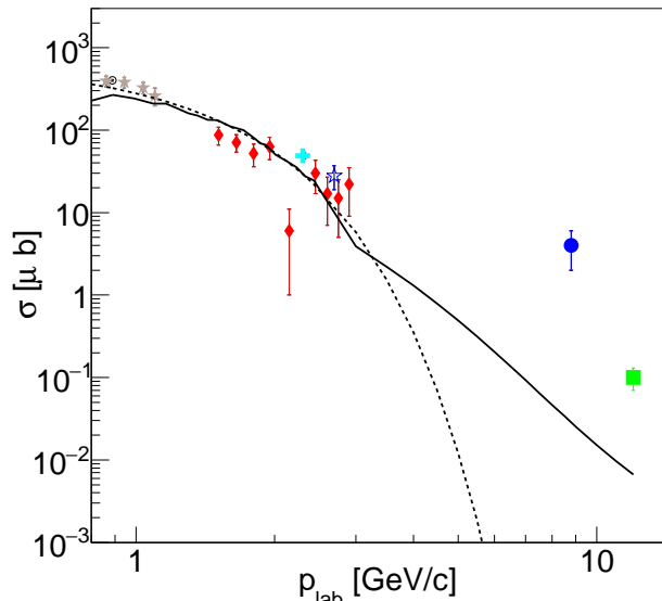
Figure 4: Total cross section for the reaction \bar{p}p \rightarrow \pi^+\pi^- , as a function of the beam momentum in the laboratory reference frame, p_{\text{lab}} . The selected data are from Refs: [12] (black open circle), [54] (blue full circle), [55] (cyan full cross), [56] (red full diamonds), [57] (brown full stars), and [58] (black open star). The result from Ref. [53] (green full square) corresponds to total backward cross section and has to be considered as a lower limit. The solid line is the result from the generator [46]. The dashed line is the result of the compilation from Ref. [45].
