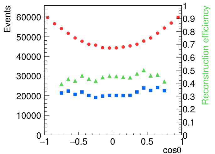
Figure 13: Angular distribution for \bar{p}p \rightarrow e^+e^- at p_{lab} = 3.3 GeV/c of generated (red circles) and reconstructed and identified (blue squares) electrons. The reconstruction efficiency (green triangles) corresponds to the y -axis scale on the right.
