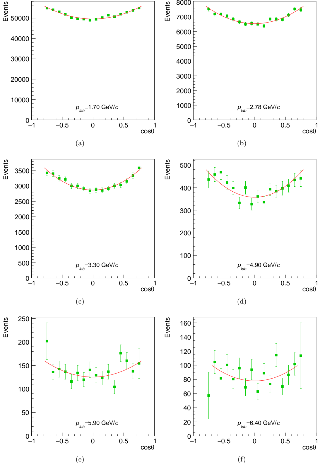
Figure 14: Reconstructed and efficiency-corrected angular distributions of generated electrons (green squares) and the fit (red line) for different p_{lab} values: (a) 1.7 GeV/c, (b) 2.78 GeV/c, (c) 3.3 GeV/c, (d) 4.9 GeV/c, (e) 5.9 GeV/c, and (f) 6.4 GeV/c.
