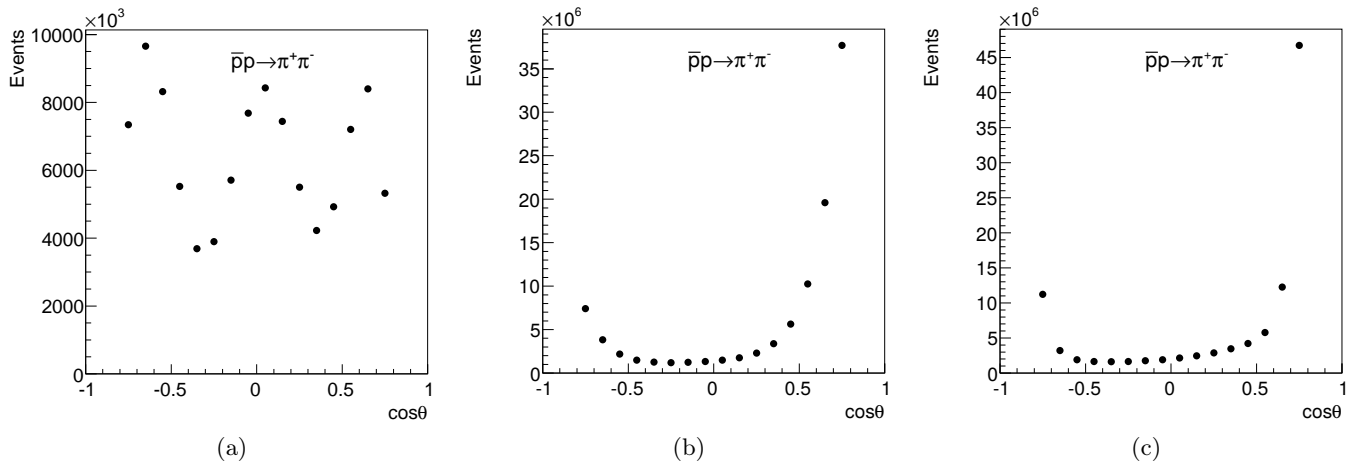
Figure 7: Angular distribution of \pi^- from the \bar{p}p \rightarrow \pi^+\pi^- events generated using the model from Ref. [46] for different p_{lab} values: (a) 1.7 GeV/c, (b) 3.3 GeV/c, and (c) 6.4 GeV/c.
