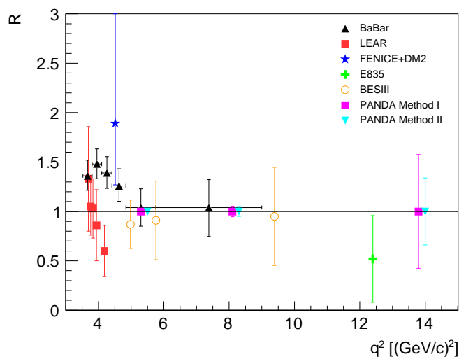
Figure 21: Expected statistical precision on the determination of the proton FF ratio from the present simulations (magenta squares and blue down triangles) for R = 1 as a function of q^2 , compared with the existing data. Data are from Ref. [12] (red squares), Ref. [13] (black up triangles), Ref. [72] (open orange circles), and Ref. [73] (green cross and blue star). The statistical uncertainties are extracted in the angular range |\cos\theta| \leq 0.8 .
