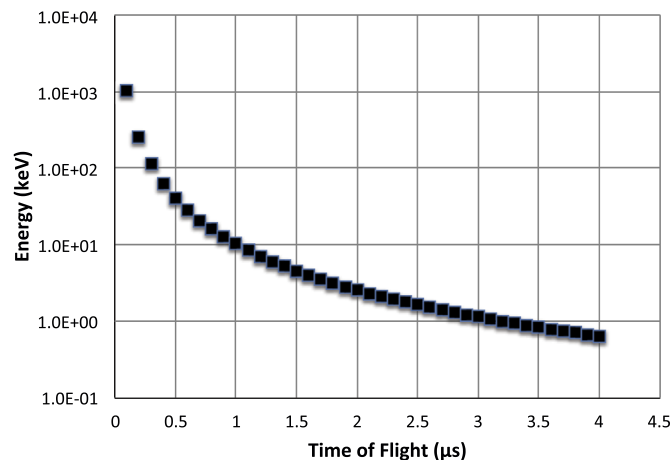
Fig. 6. Time delay vs. antiproton energy.
