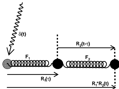
Fig. 8: Sequence of oscillators corresponding to the response function of Fig.7. In equilibrium both the black masses overlap with the grey circle. They can move horizontally under the action of elastic forces F_1 and F_2 , graphically represented as springs, or of external forces. When any of these masses is subject to an instantaneous external impulse \propto \delta(t - t_0) at the time t_0 , its later displacement from the equilibrium position is described by the Green response function R_i(t - t_0) . A short impulse by an external force \delta(t) at t = 0 causes the displacement R_1(\tau) of the first mass at the later time \tau . The displacement of the first mass acts as an external force on the second mass, and may be decomposed into short impulses: R_1(\tau) = \int d\tau' R_1(\tau')\delta(\tau - \tau') . Since each short impulse at the time \tau produces a response R_2(t - \tau) of the second mass, the resulting displacement of the second mass is \int d\tau R_2(t - \tau)R_1(\tau) .
