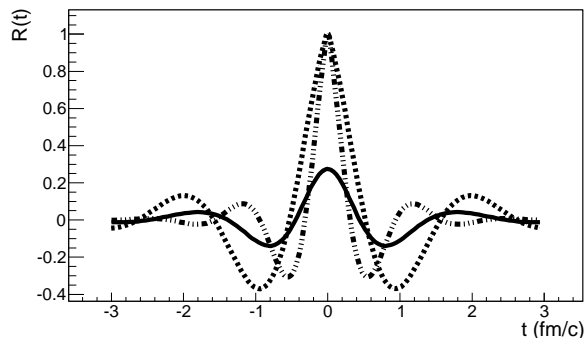
Fig. 7: Dotted line: R_1(t) = \cos(M_1 t)e^{-a|t|} , with M = 1 GeV, a = 0.4 GeV. Thick-soft double-dotted line: R_2(t) = \cos(M_2 t)e^{-b|t|} , with M_2 = 0.6 GeV, b = 0.1 GeV. Continuous line: Convolution [R_1(t) * R_2(t)] = \int d\tau R_1(\tau)R_2(t - \tau) according to eq.54.
