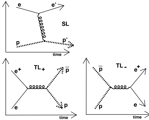
Fig. 2: Reactions 8 (labeled as SL in the figure), 8 ( TL_+ ), 8 ( TL_- ). In this work we assume single photon exchange, so that the electromagnetic form factors are functions characterizing the vertex coupling the virtual photon to the hadron current (thick grey dashed line in the figure).
