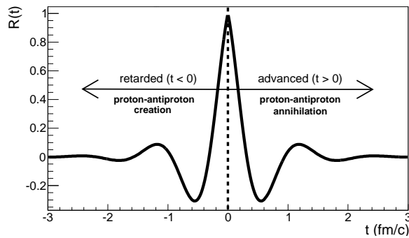
Fig. 6: R(t) = \cos(Mt)e^{-a|t|} , with M = 1 GeV, a = 0.4 GeV, as in eq.51. The retarded ( \bar{p}p creation) and advanced (annihilation) contributions of eq.52 are distinguished.
