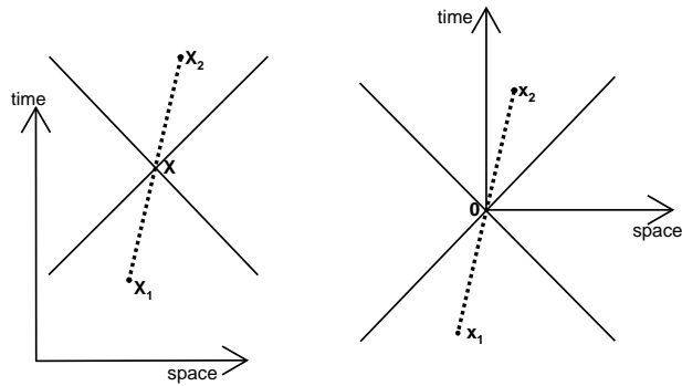
Fig. 5: Absolute (left image) and relative (right image) coordinates for the chain of events leading to \bar{p}p formation from a virtual photon as shown in Fig.4. Left image: according to eqs.33, X_1 , X and X_2 lie along a straight line, that is represented as a thick dashed line in the figure. This line does not correspond to any physical particle, we just use it to highlight the relative position of the 3 points. The continuous thin straight lines at 45^\circ and 135^\circ represent the light cone of X . Right image: the same geometry of the left image, but using the relative 4-coordinates x_1 and x_2 introduced in eqs.34. With this transformation, X becomes the origin. The 4-coordinate x that is argument of the space-time form factor F(x) coincides with x_1 , the 4-point where the photon creates the first quark-antiquark pair.
