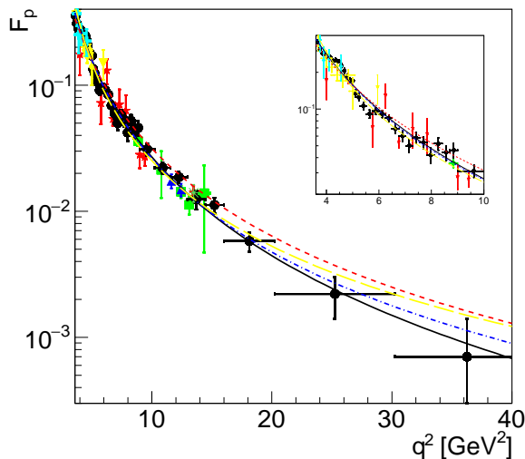
Fig. 1: World data on the TL proton generalized FF as a function of q^2 , together with the calculation from Eq. (2) (blue dash-dotted line), Eq. (3) (red dashed line), Eq. (4) (yellow long-dashed line), and Eq. 5 (black solid line). The world data are from Ref. [5, 6] (black solid circles), Ref. [7] (red stars), Ref. [8] (green squares), Ref. [9] (blue triangles up), Ref. [10] (yellow triangles down), Ref. [11, 12] (cyan full crosses), Ref. [13] (magenta full diamonds), and Ref. [14] (dark green asterisk). The insert magnifies the near threshold region.
