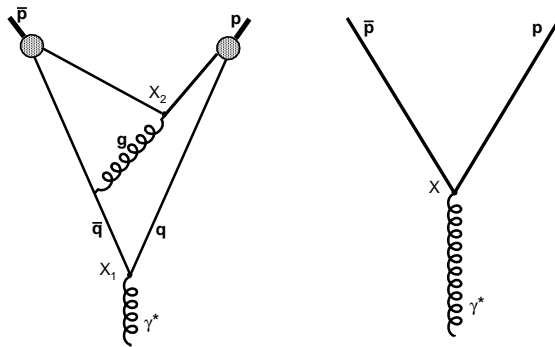
Fig. 4: Left image: one of the possible chains of events that at resolved level lead to proton-antiproton formation from a virtual photon. In this figure the proton is schematized in a simplified form, as composed by a charged quark plus a neutral compact diquark. So \gamma \rightarrow \bar{p}p requires at least 2 pair creation vertexes, in the 4-points X_1 and X_2 . Right image: the same process at unresolved level of analysis. Only one vertex is present in the 4-point X , where the \bar{p}p pair is directly created by the photon. The relation between X , X_1 , and X_2 is determined by eqs.33, that in this simple case will be of the form X = w_1X_1 + w_2X_2 . The corresponding geometry is represented in Fig.5.
