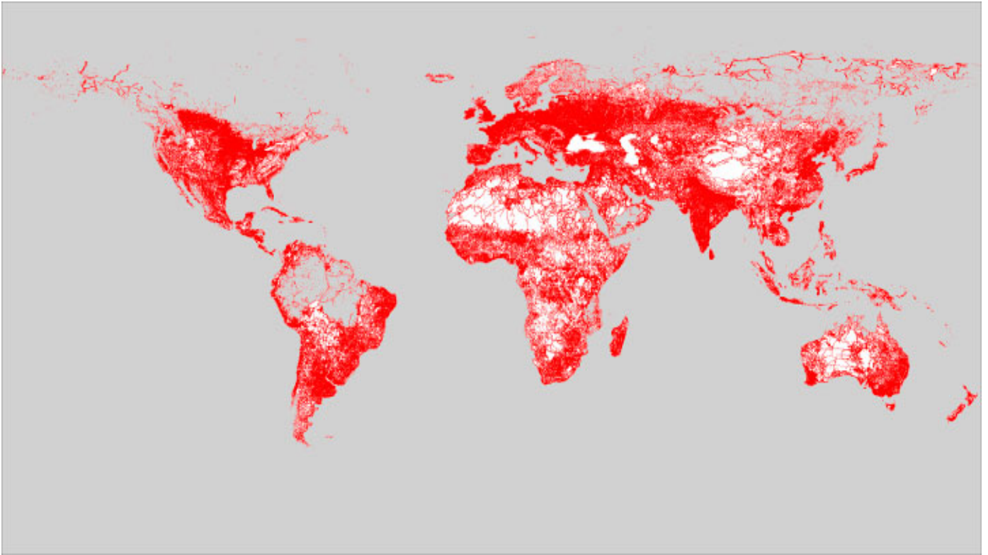
Fig. 3. Human impacted areas on the Biosphere, identified through mapping of roads, railways and settlement density (by T. Hengl ( http://globio.info ) [CC BY-SA 3.0 ( http://creativecommons.org/licenses/by-sa/3.0 )], via Wikimedia Commons).
