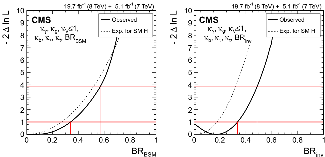
Fig. 18 (Left) Likelihood scan versus BR_{BSM} = \Gamma_{BSM}/\Gamma_{tot} . The solid curve represents the observation in data and the dashed curve indicates the expected median result in the presence of the SM Higgs boson. The modifiers for both the tree-level and loop-induced couplings are
