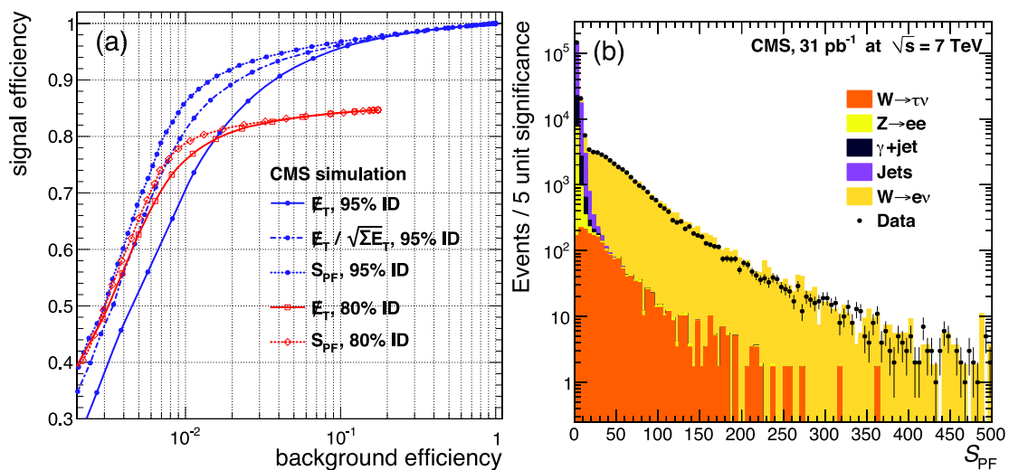
Figure 23. (left) Efficiency curves for W \rightarrow e\nu signal versus backgrounds varying the minimum value of E_T (solid lines), of S_{PF} (dotted lines), and of E_T/\sqrt{\sum E_T} (dot-dash line), with the 95% efficient (blue) or 80% efficient (red) electron isolation criterion applied. (right) Distributions of S_{PF} in candidate W \rightarrow e\nu events from data (points) and simulation (stacked histograms). The simulation components, from top to bottom, are signal (mustard) and backgrounds from jets (purple), \gamma +jets (black), Z \rightarrow e^+e^- (yellow), and W^\pm \rightarrow \tau^\pm\nu_\tau (orange). The simulation is scaled by a fit to the data with floating normalizations for the signal and the total background.
