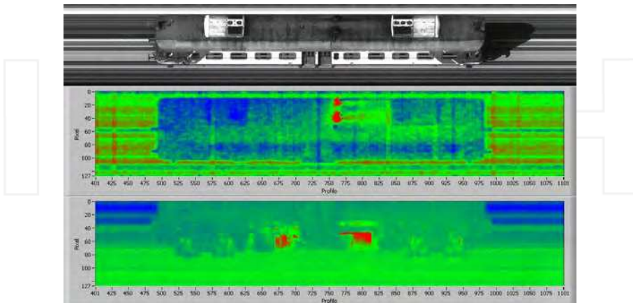
Fig. 5. Example of the acquisition of the left side of a locomotive concurrently performed by the upper image acquisition system, and the upper and lower thermal monitoring systems.
