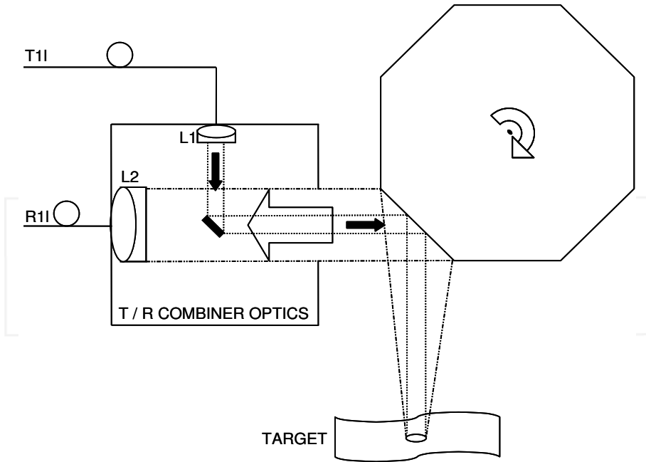
Fig. 10. Optical layout of the remote station, with polygonal mirror and T/R combiner optics.
