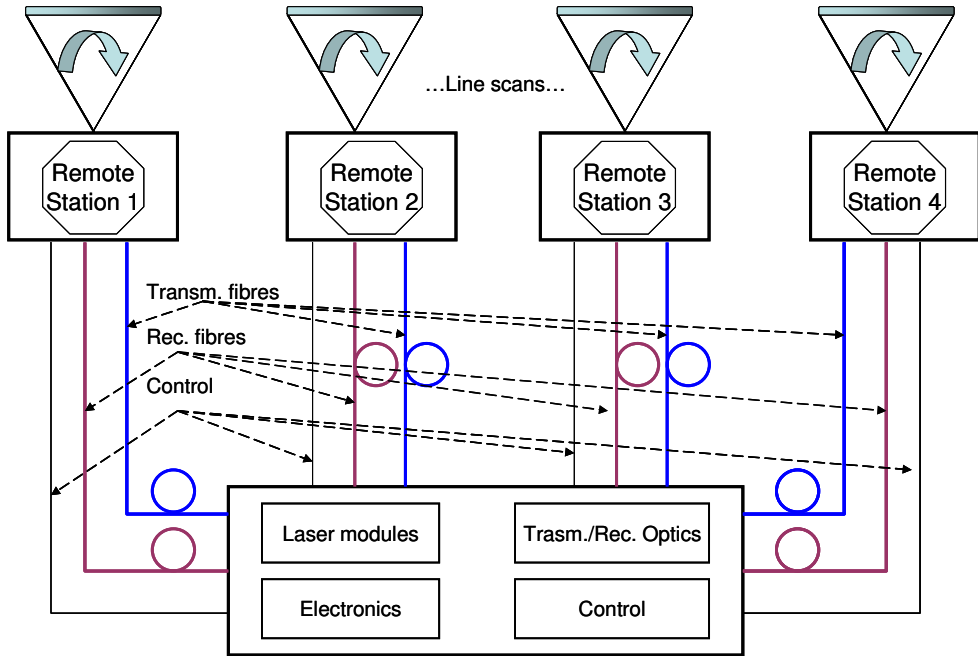
Fig. 7. Overall layout of the telemeter.
