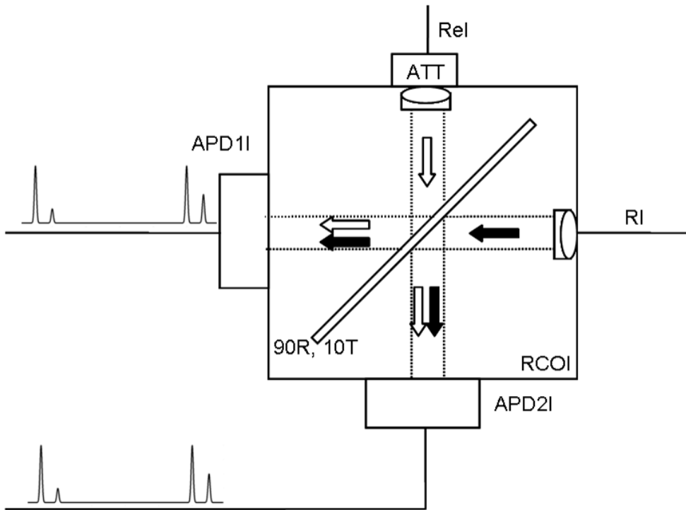
Fig. 9. Detail of the receiver collimation optics (RCO).
