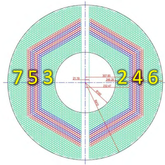
Figure 6.18: The numbers correspond to the different sectors in which the STT is divided. 2 and 3 are inner parallel tubes, 4 and 5 are skewed tubes and 6 and 7 are outer parallel tubes.
