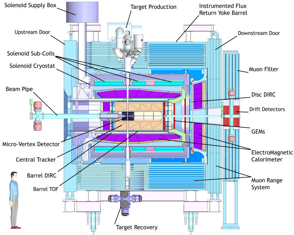
Figure 1.9: Artistic side view of the Target Spectrometer (TS) of \bar{P} ANDA. To the right of this the Forward Spectrometer (FS) follows, which is illustrated in Fig. 1.13.
