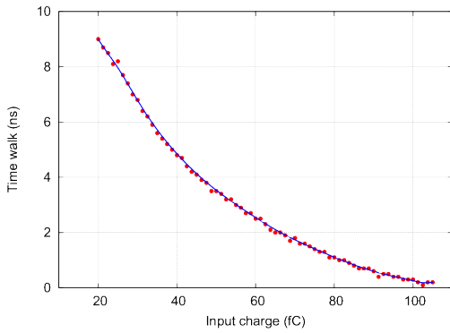
Figure 3.7: Example measurement of the discriminator time walk.
