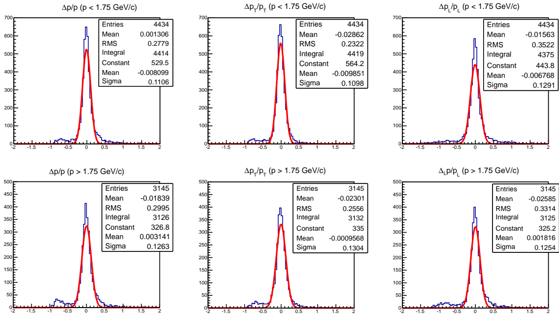
Figure 6.20: \frac{\Delta p}{p} = \frac{RECO_p - MC_p}{MC_p} for the protons and antiprotons which form the \Lambda and \bar{\Lambda} of Fig. 6.19. The first column plots the total momentum, the second column the transverse momentum and the third column the longitudinal momentum. The two rows represent the low momentum (top) and high momentum (bottom) particles.
