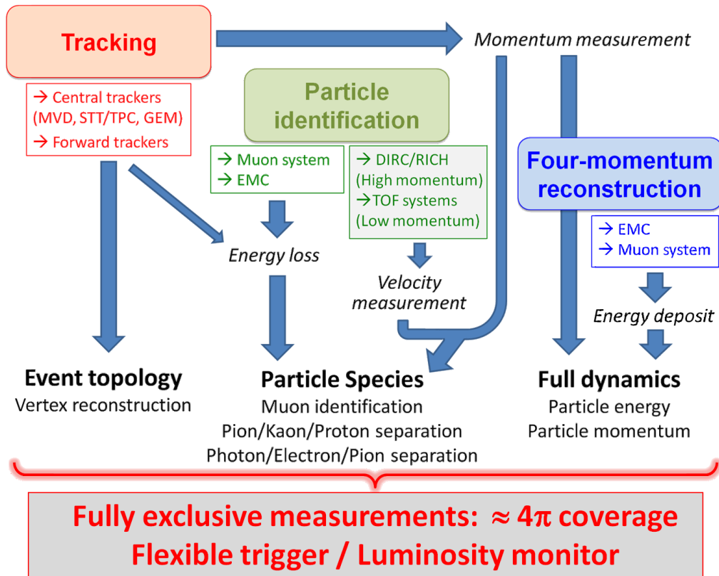
Figure 1.8: Basic detection concept. The main components are described in sections 1.2.1 and 1.2.2.
