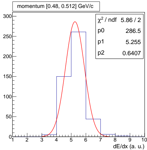
Figure 6.27: Example of a dE/dx truncated mean distribution for muon tracks with momentum in the range [0.48, 0.512] GeV/c: it shows a Gaussian shape as expected.
