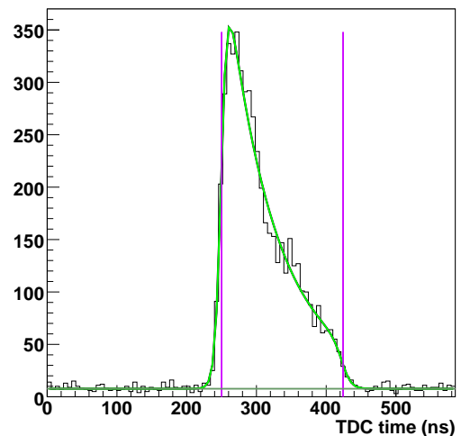
Figure 4.2: Example of a fitted TDC spectrum. The light green line is the fit of the distribution; the violet vertical lines correspond to the t_0 and t_{max} values determined by the fit. The dark green horizontal line indicates the noise level.
