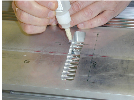
Figure 2.11: Gluing of straw tubes to multi-layers.
