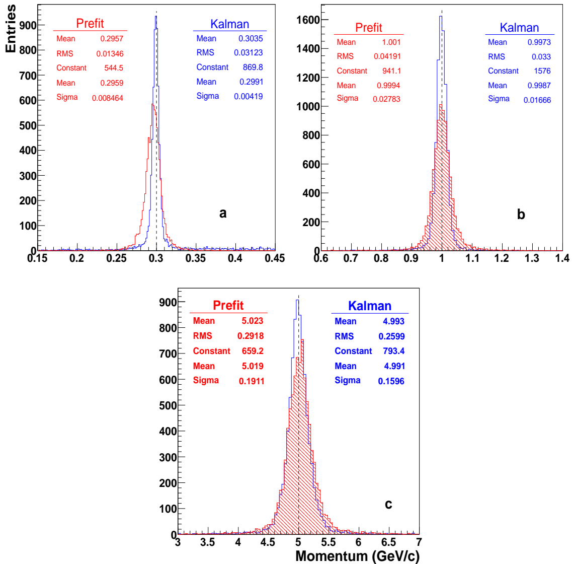
Figure 7.5: Momentum distributions for (a) 0.3, (b) 1 and (c) 5 GeV/c \mu^- , reconstructed with helix (red dashed) and Kalman (blue) fits. The statistic boxes report the mean values and RMS of the non fitted histograms, as well as mean and sigma values of the Gaussian fits, before and after the Kalman fit.
