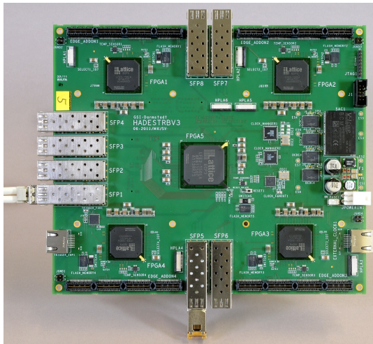
Figure 3.16: Produced TRBv3 board.
