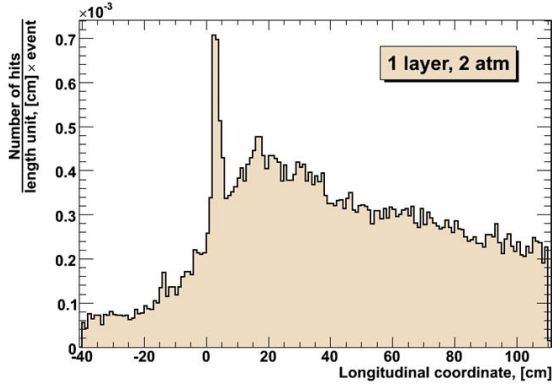
Figure 5.24: Simulation of \bar{p}p reactions giving the number of hits per event and per cm along the tubes in the innermost layer of the PANDA straw tube tracker. The target position is at z=0 cm.
