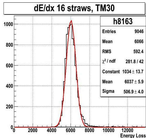
Figure 5.12: dE/dx distribution for 2.95 GeV/c protons fitted with a Gaussian curve. The protons hit 16 straw tubes, and a truncation of 30% has been applied.
