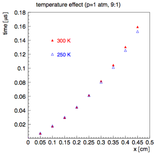
Figure 2.6: Space time relation for the Ar+10% CO 2 mixture at 1 atm for two different temperatures.
