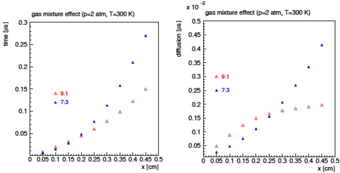
Figure 2.5: The graphs refer to two gas mixtures with different CO 2 percentage. Red points correspond to a percentage of 10% of CO 2 , blue to 30%.
