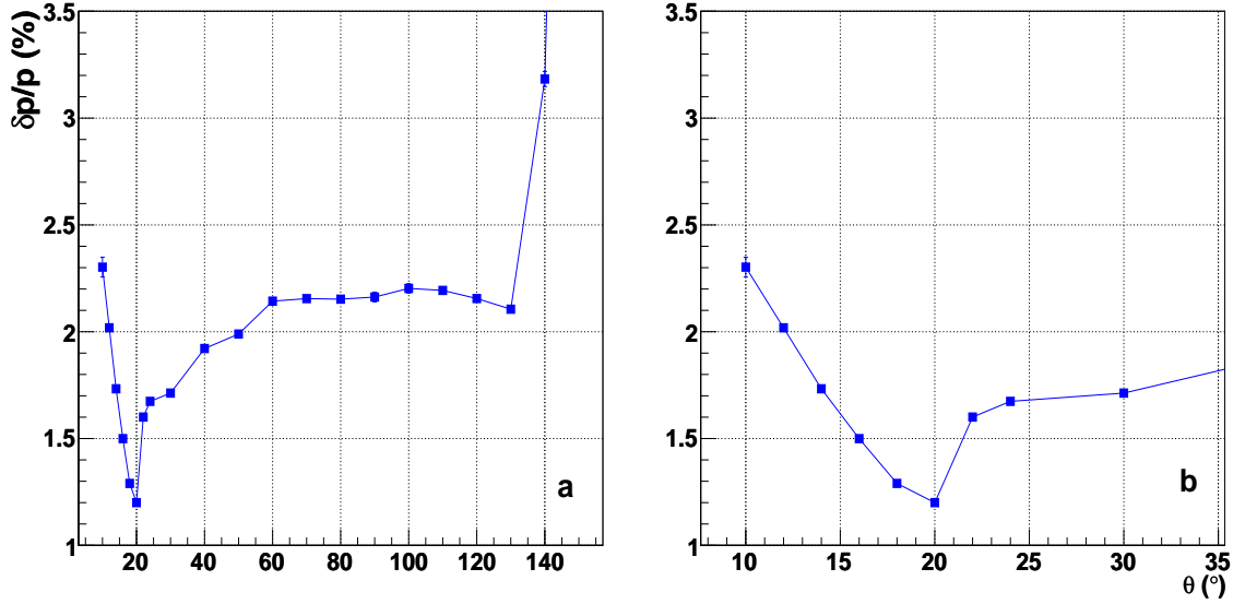
Figure 7.10: Momentum resolution vs. \theta starting angle for 2 GeV/c \mu^- single track events, in the full angular range \theta \in [9^\circ, 160^\circ] (a) and in the forward region \theta \in [9^\circ, 35^\circ] (b) (see Table 7.4).
