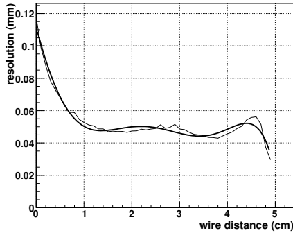
Figure 6.12: As in Fig. 6.11 with a constant fraction electronic discrimination.
