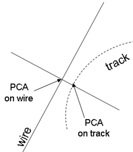
Figure 6.23: Sketch of the positions of the point of closest approach (PCA) on the track and on the wire.
