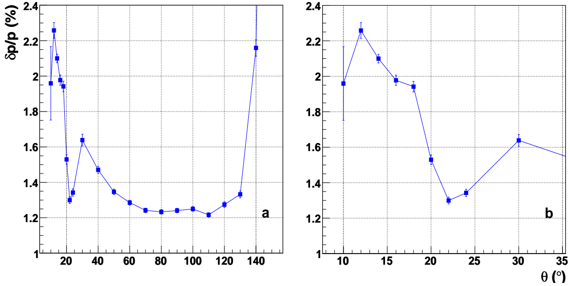
Figure 7.6: Momentum resolution vs. \theta starting angle for 0.3 \text{ GeV}/c \mu^- single track events, in the full angular range \theta \in [9^\circ, 160^\circ] (a) and in the forward region \theta \in [9^\circ, 35^\circ] (b) (see Table 7.2).
