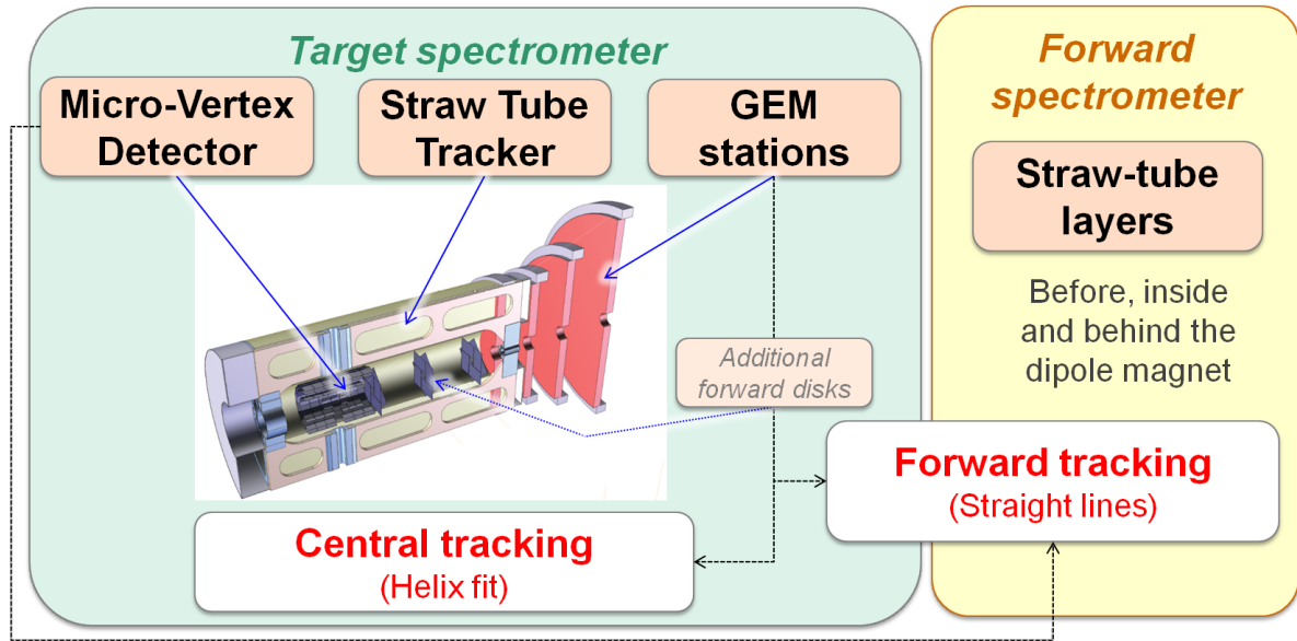
Figure 1.15: Overview of the \bar{P} ANDA tracking system, including the option of the additional forward disks.
