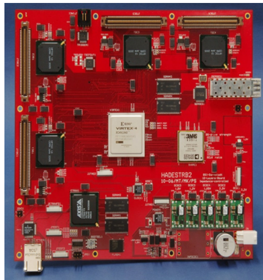
Figure 3.18: HADES TRBv2 board.
