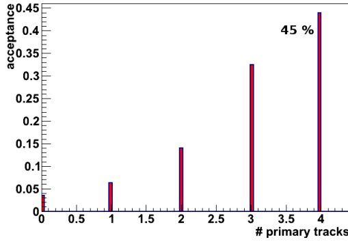
Figure 7.37: Multiplicity of the kaons from the reaction \eta_c \rightarrow \phi\phi \rightarrow K^+K^-K^+K^- within central tracker acceptance.
