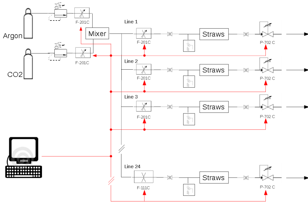
Figure 2.23: Scheme of the gas system.
