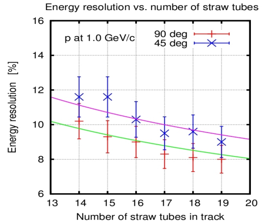
Figure 5.17: Dependence of the energy resolution on the number of hit straws for protons with 1.0 GeV/c momentum. For the setup inclined by 45^\circ the resolution is slightly worse, from about 8% to 9% at 19 hit tubes.
