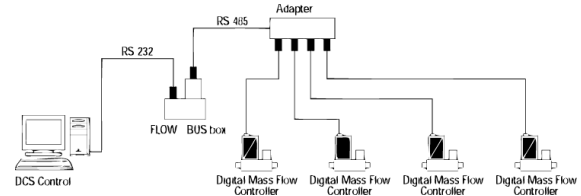
Figure 3.20: Layout of the STT gas control system.
