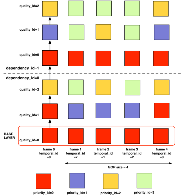
Figure 1: Example of priority_id assignment for two spatial resolutions.
