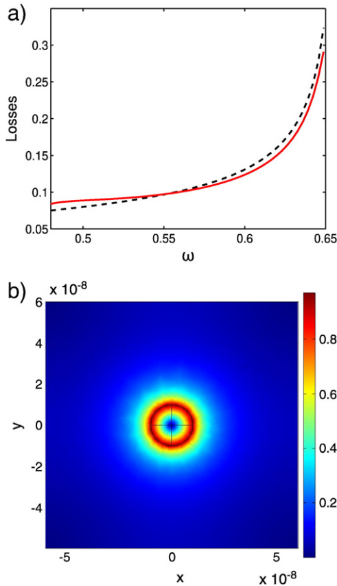
Fig. 5. In a) the comparison is shown between losses \gamma_I calculated as imaginary part of k obtained by numerically solving Eq. (2) (red lines) and losses \gamma_{pl} predicted by Eq. (18) (black dashed lines). In b) the longitudinal mode at \omega=0.5 is shown (norm of the magnetic field).
