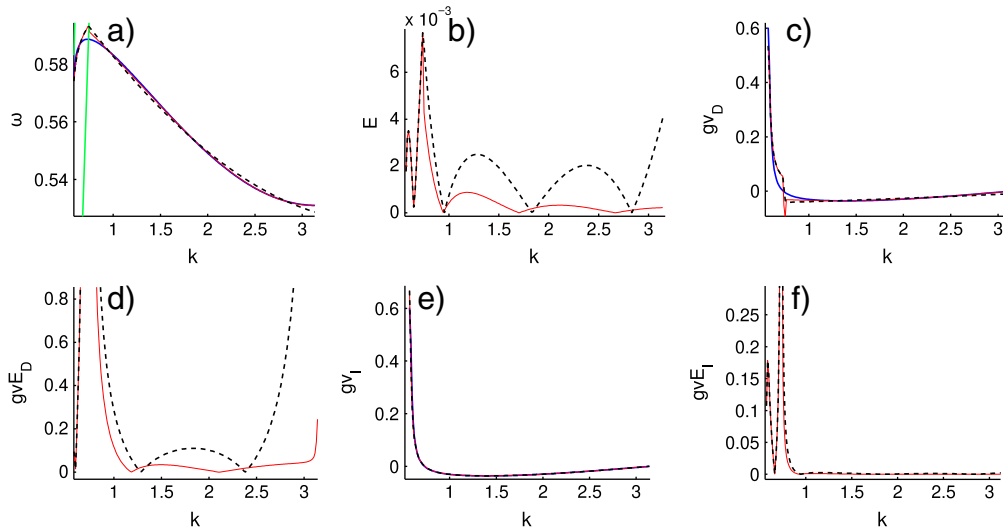
Fig. 4. Same as Fig. 3, but the transverse mode is analyzed. Blue lines in a), c) and e) represent the exact numerical results; red lines the approximated results obtained by interpolating F_I with F_{I1} in R_{I1} and F_{I2} in R_{I2} . Region R_{I1} is between the two green lines in a), the first of whom on the left is the light one.
