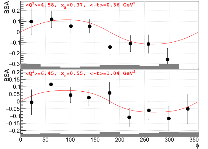
Fig. 5. Beam spin asymmetry as a function of \phi for two representative kinematic bins. The vertical error bars show the statistical uncertainty of each point. The gray bands represent systematic uncertainties of the BSA measurements. The red lines show the fit with functional form of Eq. (1).
