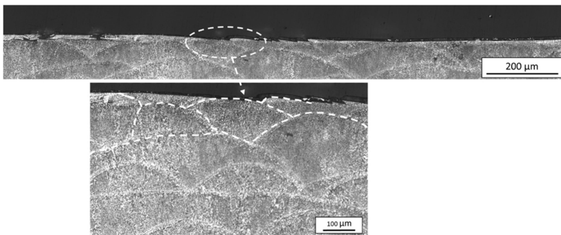
Figure 9. Cross sections of as-produced AM-xy sample after 10 m sliding distance.
