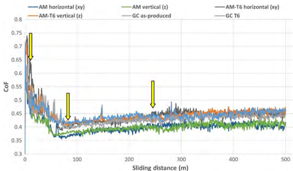
Figure 6. CoF tendency with sliding distance. Arrows indicate the distance chosen for shorter tests and SEM analysis.
