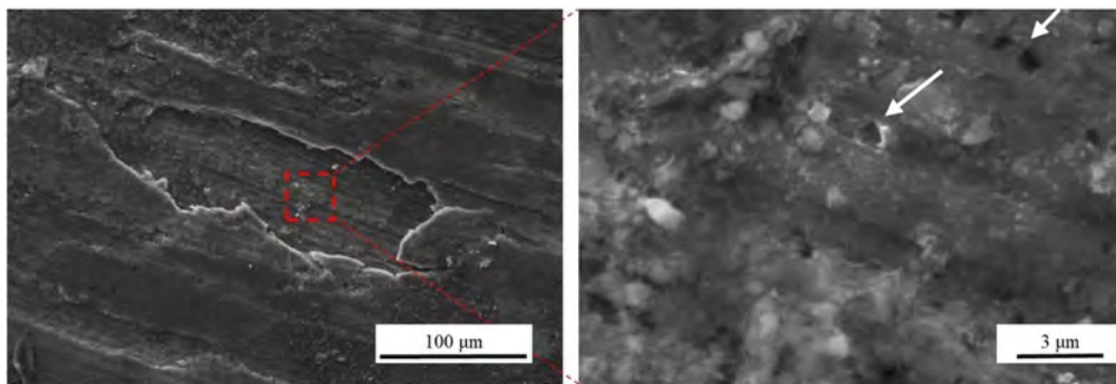
Figure 14. SEM images. Details of the worn surface after 250 m for the AM-T6 xy sample.
