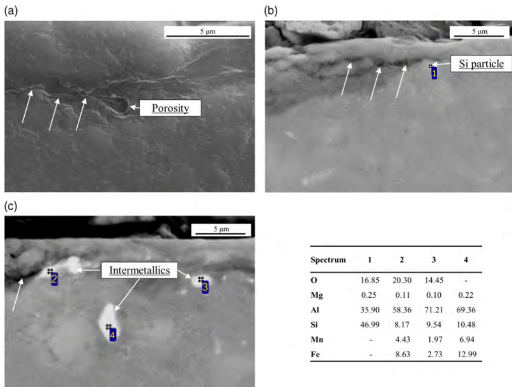
Figure 16. Particulars of cross-section SEM images and EDS analysis of the wear track at the end of the test for samples: a) AM-z, b) AM T6-z, and c) GC T6.
