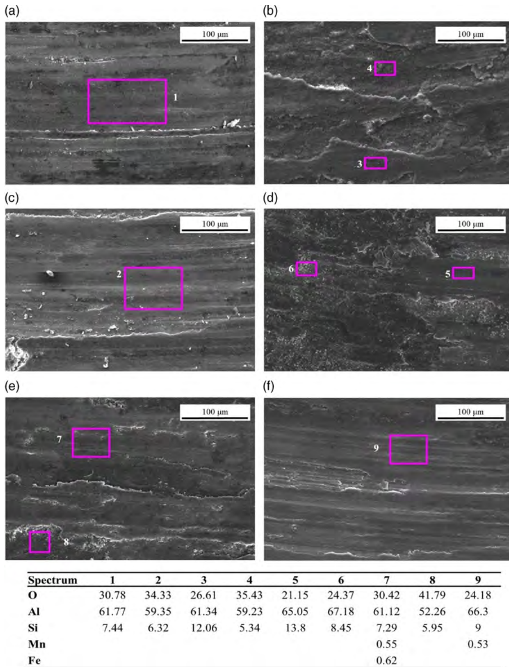
Figure 12. SEM images of wear tracks after 250 m testing for samples: a) AM-xy, b) AM T6-xy, c) AM-z, d) AM T6-z, e) GC, and f) GC T6.
