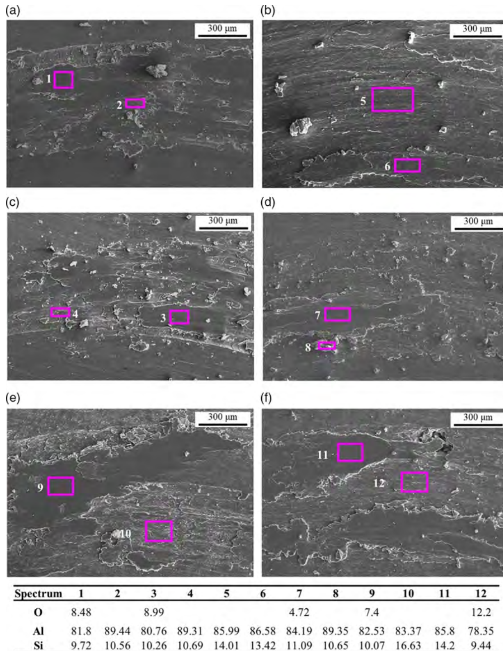
Figure 8. SEM images of wear tracks after 10 m testing for samples a) AM-xy, b) AM T6-xy, c) AM-z, d) AM T6-z, e) GC, and f) GC T6.
