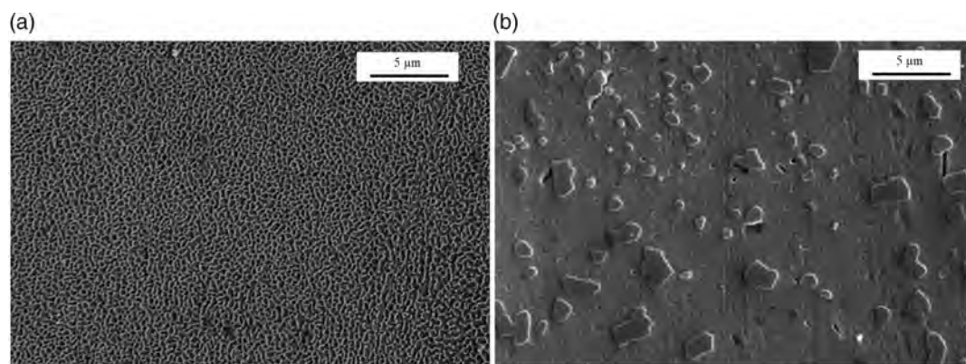
Figure 3. SEM image of a) AM as-produced and b) AM T6 sample.
