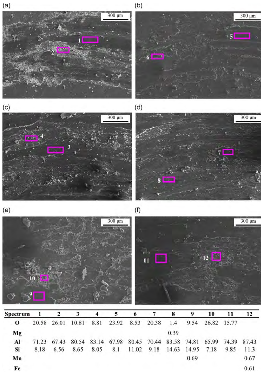
Figure 11. SEM images of wear tracks after 80 m testing for samples: a) AM-xy, b) AM T6-xy, c) AM-z, d) AM T6-z, e) GC, and f) GC T6.
