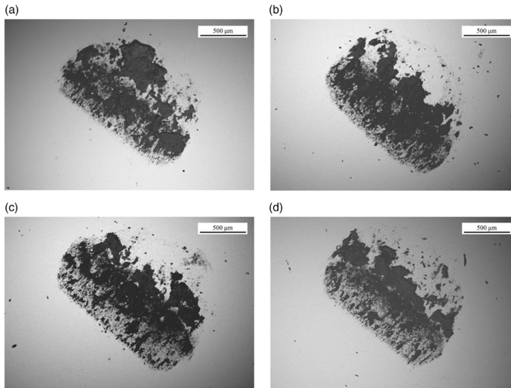
Figure 13. SEM images of the 100Cr6 ball contact area at the end of the tests for samples: a) AM-z, b) AM T6, c) GC, and d) GC T6.
