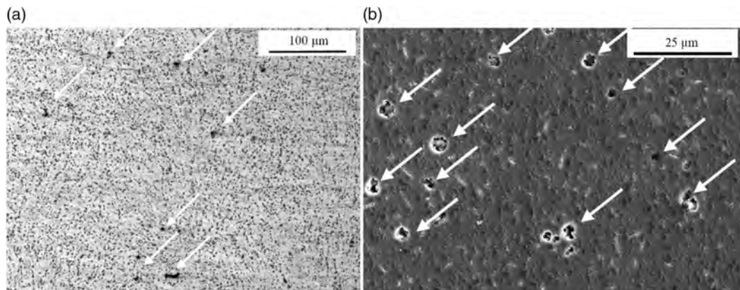
Figure 2. a) Microstructure and b) SEM image of AM samples after T6 treatment. White arrows indicate small pores.
