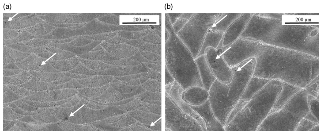
Figure 1. AM as-produced samples: a) vertical and b) horizontal cross section. White arrows show evidence of small pores.
