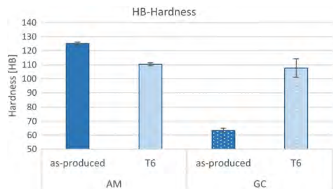
Figure 5. Brinell hardness values of studied samples. [30]
