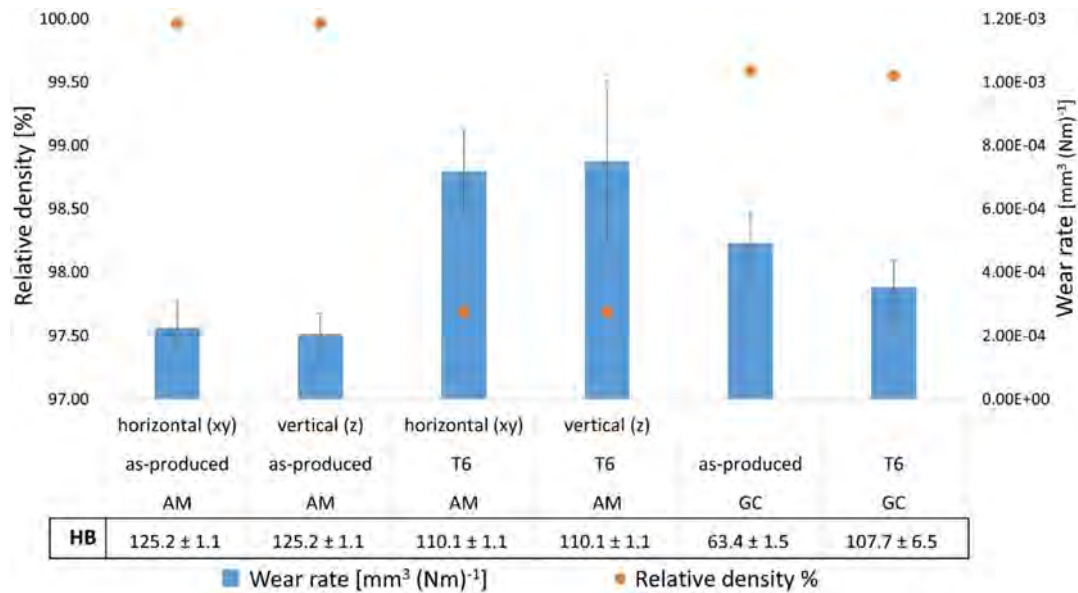
Figure 7. Wear rate ( \text{mm}^3 \text{N}^{-1} \text{m}^{-1} ) after 500 m distance of the tested samples versus hardness and relative density values.
