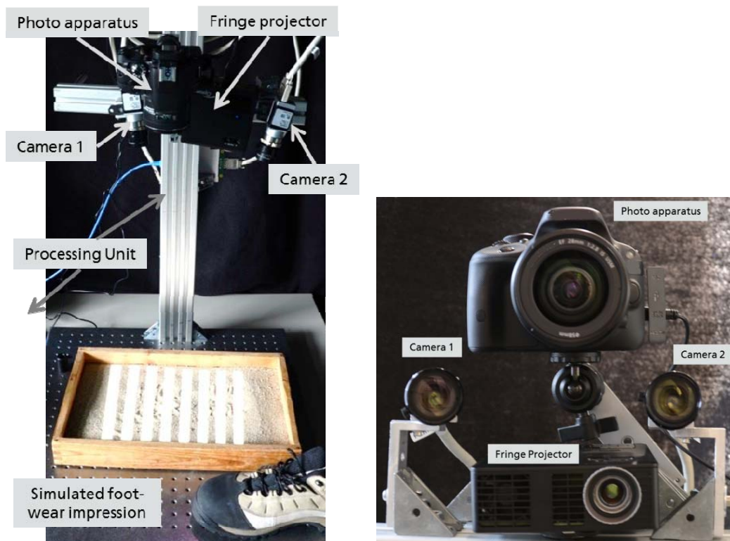
Fig. 4: Laboratory realization of the new 3D-Forensics handheld scanning system
