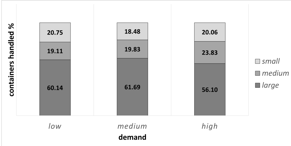
Figure 16: Percentage of containers transhipped for each terminal size for different levels of demand
