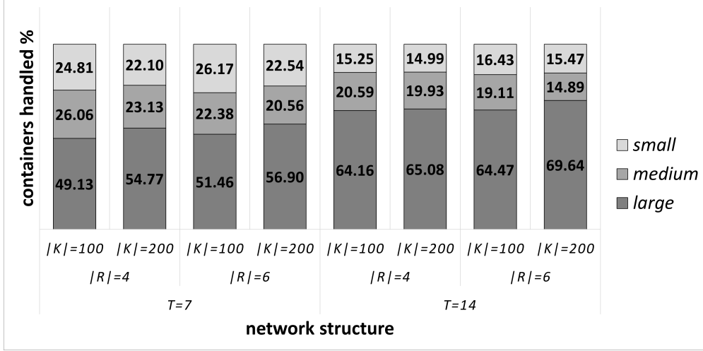
Figure 15: Percentage of containers transhipped for each terminal size for different numbers of regions, commodities, and periods
