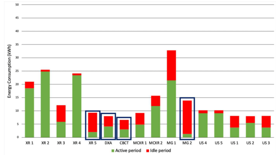
Figure 4. Energy usage for each imaging modality (active period and idle period during a working day). Modalities with high energy waste during idle period are contoured with dark blue boxes.
