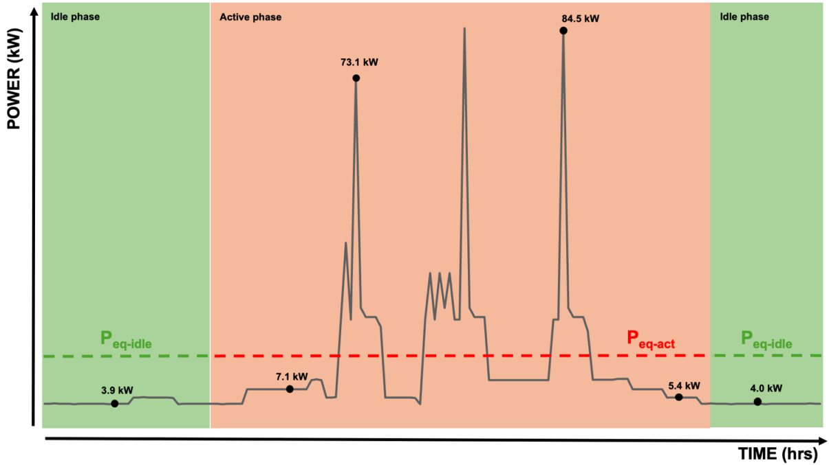
Figure 3: Diagram showing the representation of a CT scan is segmented (orange area) according to scan time. The equivalent mean power demand represents the average power required by the scanner during the active phase, considering power peaks during scanning and low power phases. The black dots on the power consumption diagram exemplify the consumption in kilowatts at the respective position on the graph. The green area identifies the waiting phase and defines the area associated with the equivalent mean power demand of that phase.
