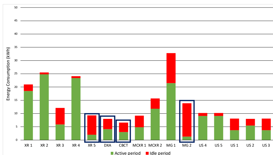
Figure 15: Energy usage for each imaging modality (active period and idle period during a working day). Modalities with high energy waste during idle period are contoured.
