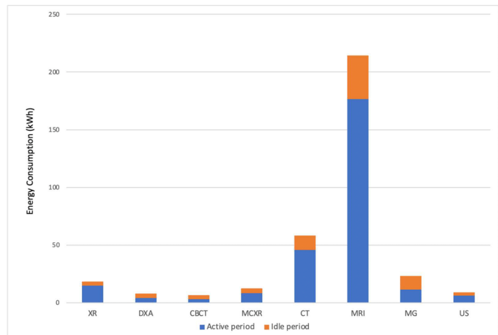
Figure 5. Mean energy consumption (kWh) for each imaging modality (active period and idle period during a working day).
