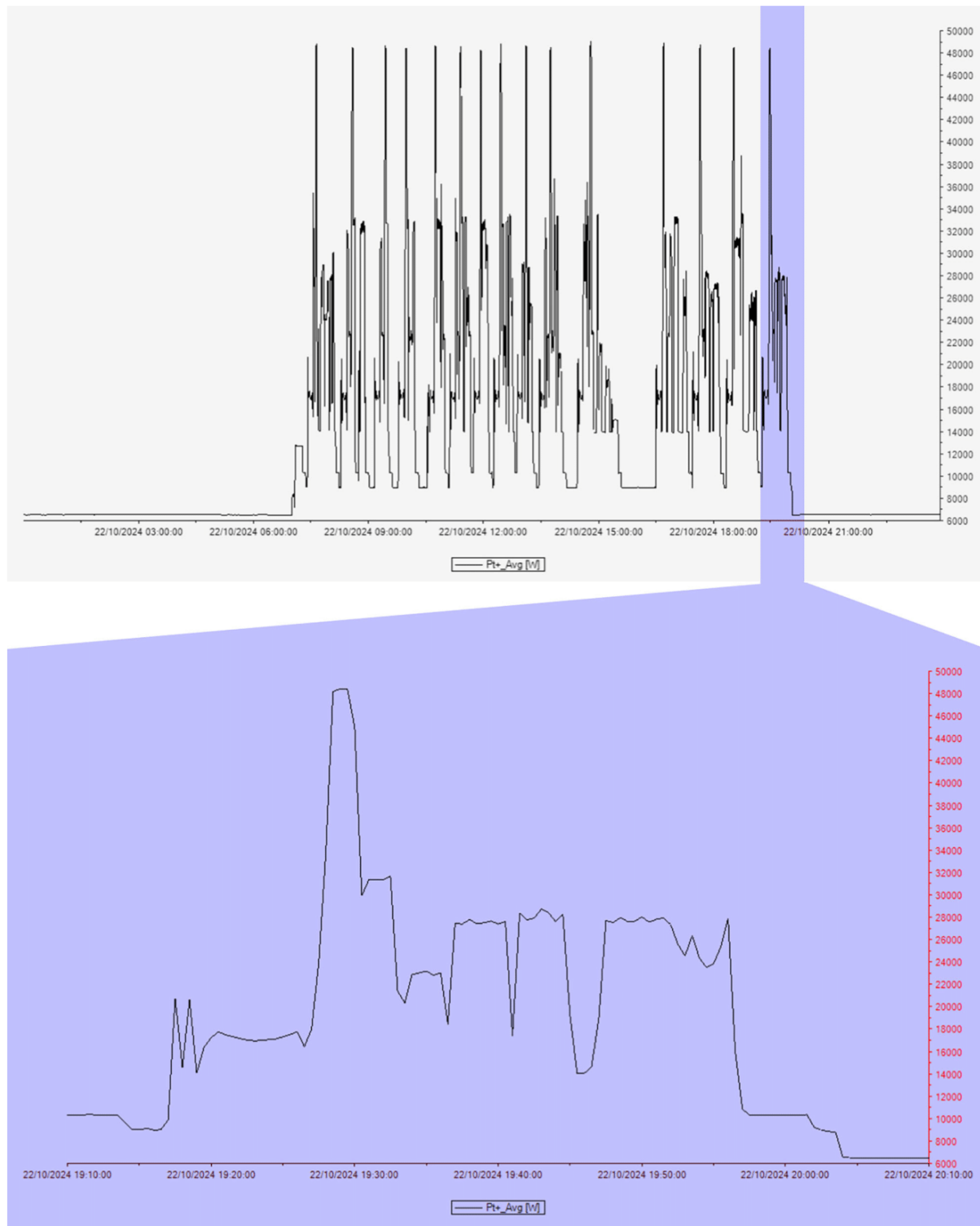
Fig. 3 The graphs show the consumption profile (in W) of an MRI unit working day recorded by the power quality analyzer, in which an MRI scan is zoomed in to show the footprint of energy consumption in the active state
