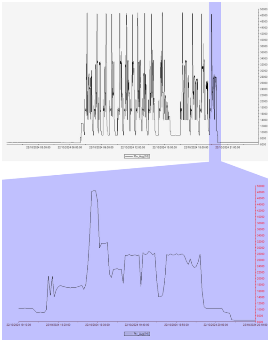
Figure 6: The figure shows the consumption profile in watts (W) of an MRI working day recorded by the power quality analyser in which an MRI scan is zoomed in to show the footprint of energy consumption in the active state.
