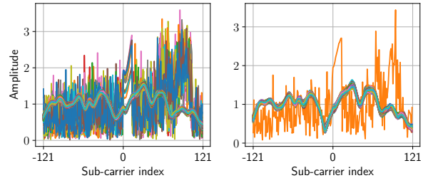
Figure 6: CSI samples from the dataset in [12] before filtering the spurious data.
