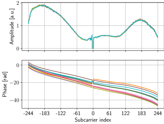
Figure 1: Amplitude (top) and phase (bottom) of 10 different CSI collected during a 10-minute experiment (code E40.0/0, see Tab. I). Amplitude values are normalized by the integral of the energy to remove the effect of the AGC.
