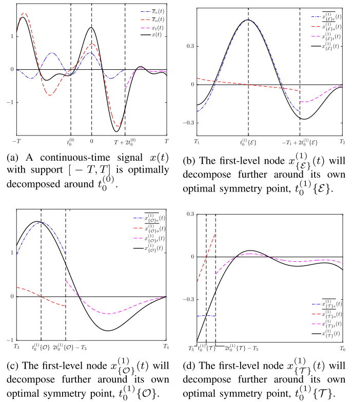
Fig. 4. First-level ternary decomposition of a sample signal x(t) . Temporal extents T_i are reported without further explanation of their inter-relationships for simplicity. The even node x_{\{\mathcal{E}\}}^{(1)}(t) of Fig. 4(b) is the causal part of the blue signal of Fig. 4(a) in the [t_0^{(0)}, T + 2t_0^{(0)}] interval; the odd node x_{\{\mathcal{O}\}}^{(1)}(t) of Fig. 4(c) is the anticausal part of the red signal of Fig. 4(a) in the [-T, t_0^{(0)}] interval; the tail node x_{\{\mathcal{T}\}}^{(1)}(t) of Fig. 4(d) is the magenta signal of Fig. 4(a) in the [T + 2t_0^{(0)}, T] interval.
