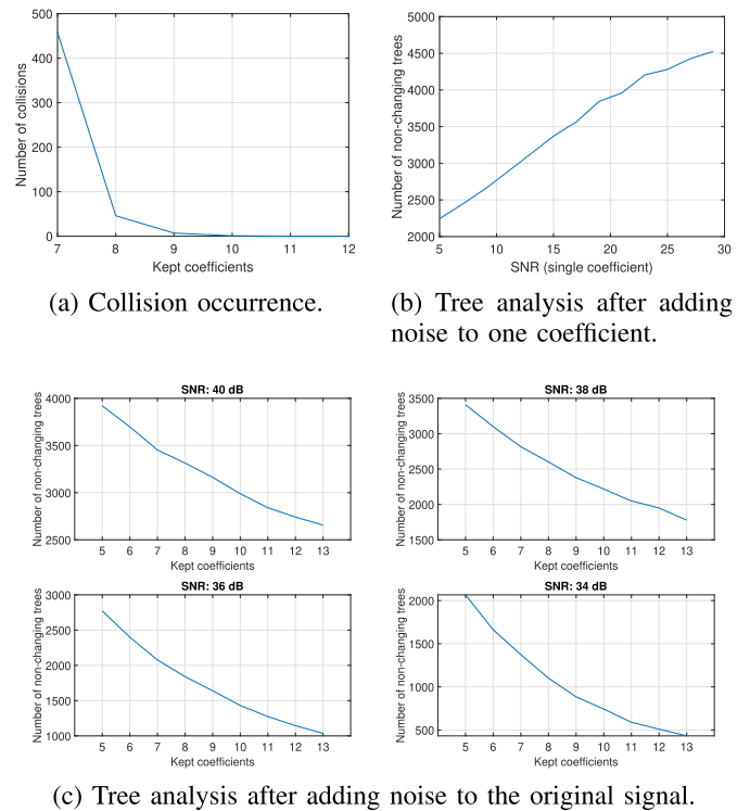
Fig. 10. Experiments on one-wayness property.
