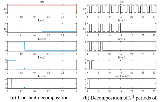
Fig. 6. Exemplification of the single branch tree property. Just the first 4 levels are shown. Each level is represented by concatenating the node signals at that level. The fourth level in Fig. 6(b) converges to p(t) in Fig. 6(a) except for a constant. (a) Constant decomposition. (b) Decomposition of 2^4 periods of p(t) . Level 4 converges to 4p(t) .
