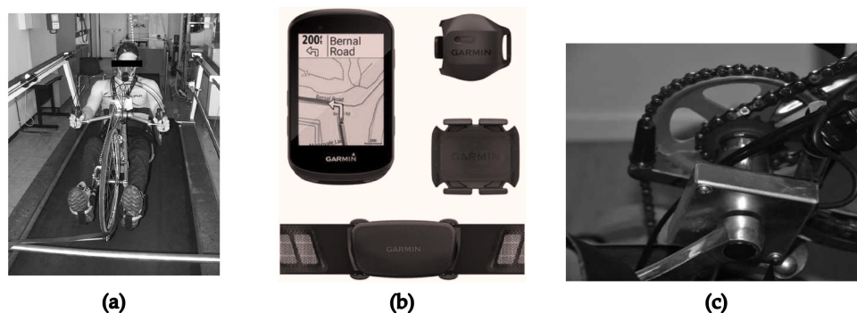
Figure 18. Examples of sensors used in the experimental setup of documents in the sensors category: from the left, (a) a spirometer used in V02 measurements (source: Abel et al., 2006 [1]), (b) a bike computer, a cadence sensor, and an HR sensor (source: Koontz et al., 2021 [65]), and (c) an encoder mounted on a handbike (source: Bakkum et al., 2014 [41]).
