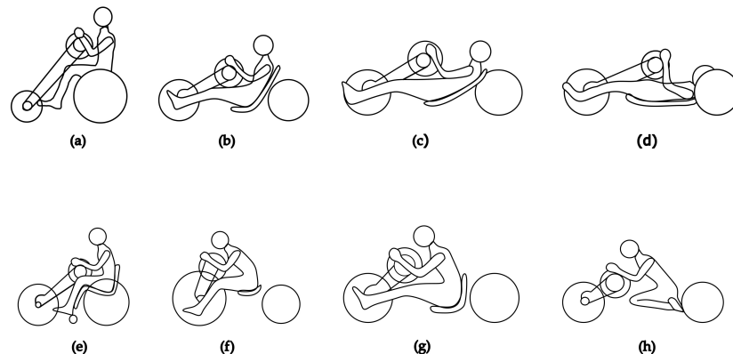
Figure 1. Schematic of the most common kinds of handbike architectures, divided into arm propulsion on the upper row, and arm trunk propulsion on the lower row, with: (a) attach unit handbike, (b) recumbent 60° rigid frame, (c) recumbent 30° rigid frame, (d) recumbent 0° rigid frame, (e) attach unit handbike, (f) car-seat, (g) long-seat, and (h) knee-seat.
