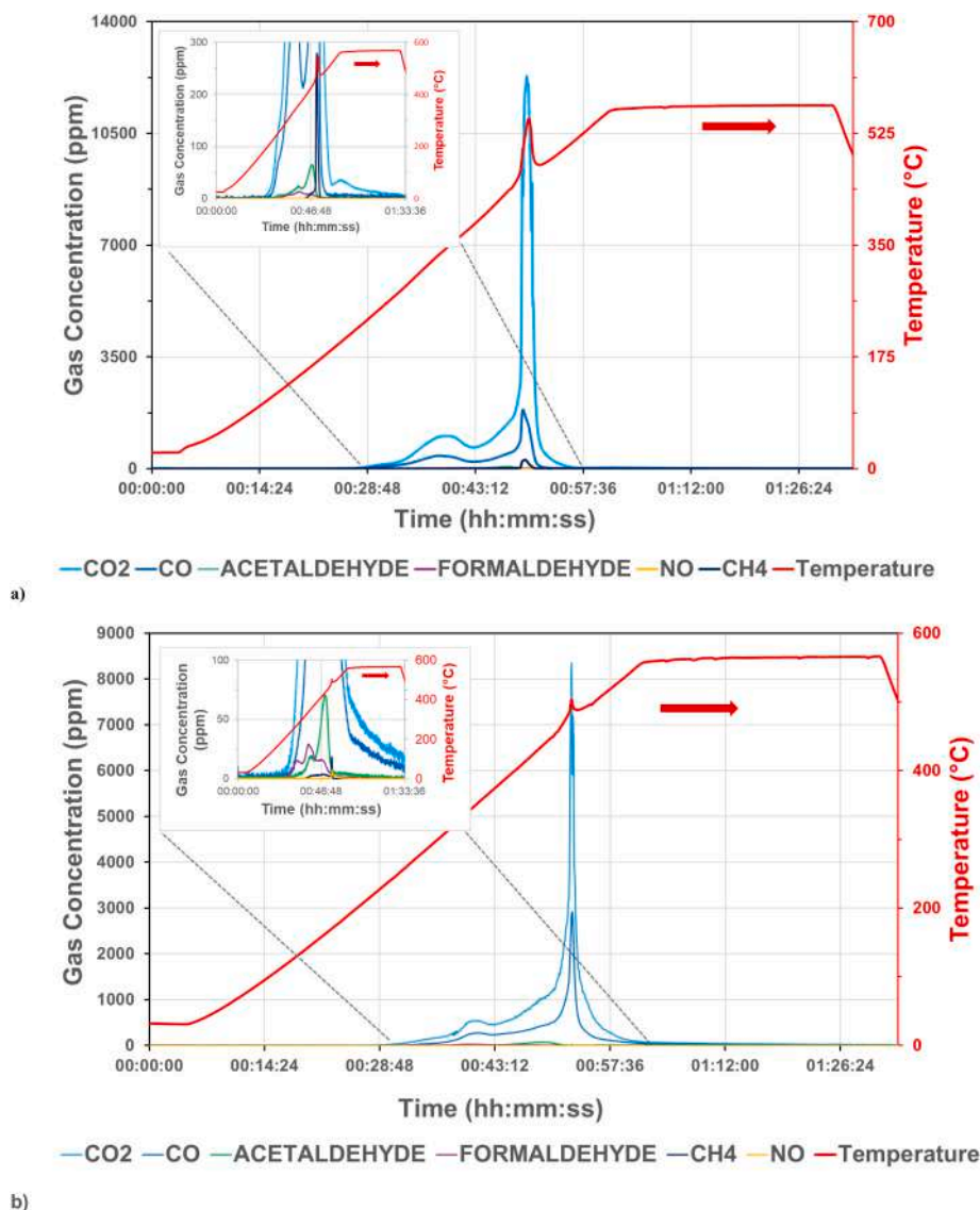
Fig. 17. TPO profiles obtained for materials a) K30, b) K70, and c) K340, during the TPO experiments. The CO 2 , CO and other gases concentration (ppm, left axis) detected during the thermal decomposition of the material and the temperature profile (°C right axis) are plotted as a function of reaction time. In the inset of the enlargement the gases evolved in low concentrations.
