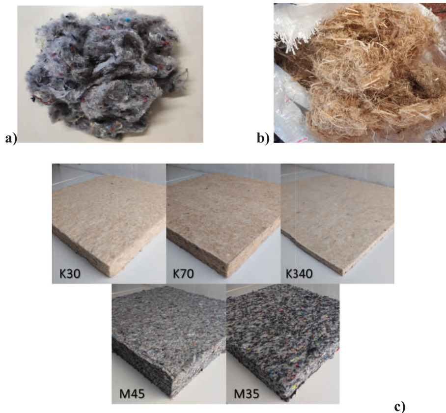
Fig. 1. Materials analyzed in this study: (a) recycled textile fibers used to produce M-type panels; (b) a mix of kenaf and hemp fibers used for the fabrication of K-type panels. These raw materials are processed by the manufacturer to obtain the final insulation panels (c). Specimens analyzed: K30, K70, and K340 panels are composed of kenaf and hemp fibers, while M45 and M35 panels are made of recycled textile fibers. All panels contain polyester as a binding agent.
