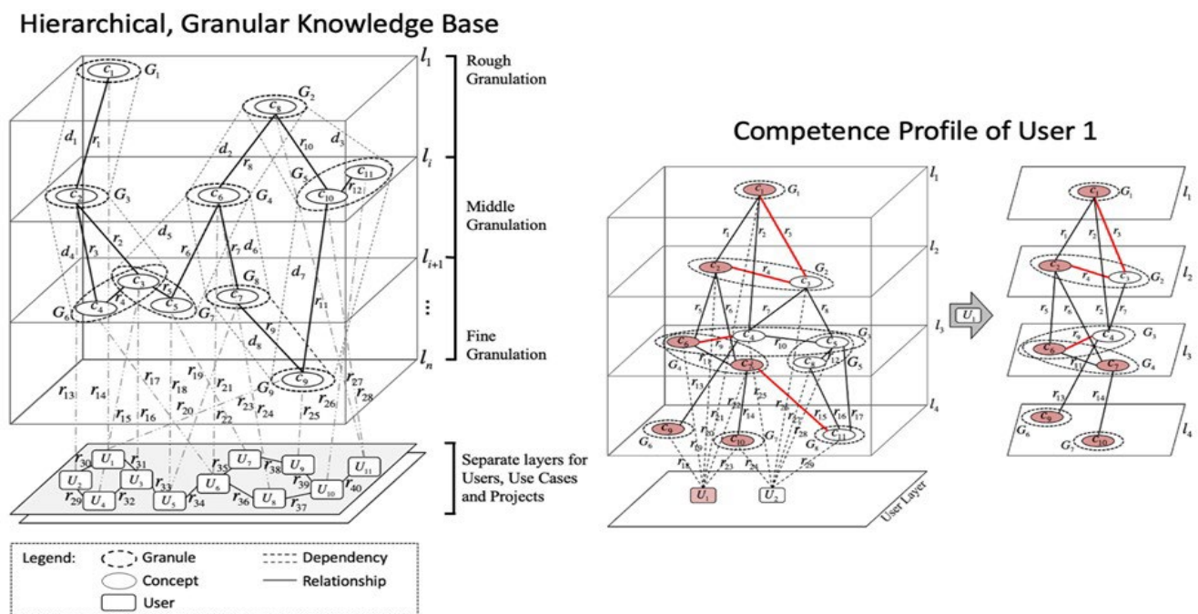
Figure 6: Hierarchical, granular Knowledge Base
