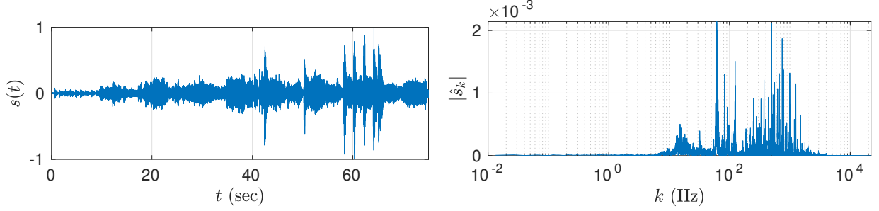
Figure 1: The signal s(t) of the 'Dance of the sugar plum fairy' in the Nutcracker of Tchaikovsky (on the left) and its Fourier spectrum (on the right).
