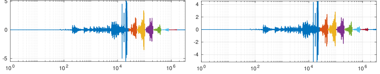
Figure 3: Two wavelet spectra (12) relative to the signal s(t) plotted in Fig. 1, computed with Daubechies wavelets (on the left) and with Haar wavelets (on the right). In both cases the blue part refers to the approximations coefficients \hat{c}_{j_0,k} , while the other coloured parts refer to the detail coefficients \hat{d}_{j,k} , different colours refer to different scale indexes j = j_0, \dots, J .
