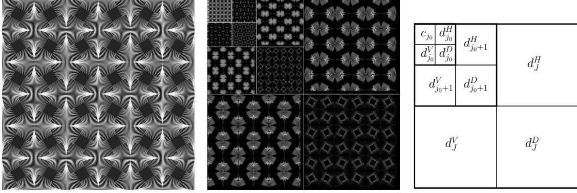
Figure 5: Marcello Morandini's pannello 593/2012. The original image (left) and its two-dimensional DWT transform (middle) with three scales: j_0 , j_0+1 and J = j_0+2 . On the right, the description of the coefficients shown in the middle image.
