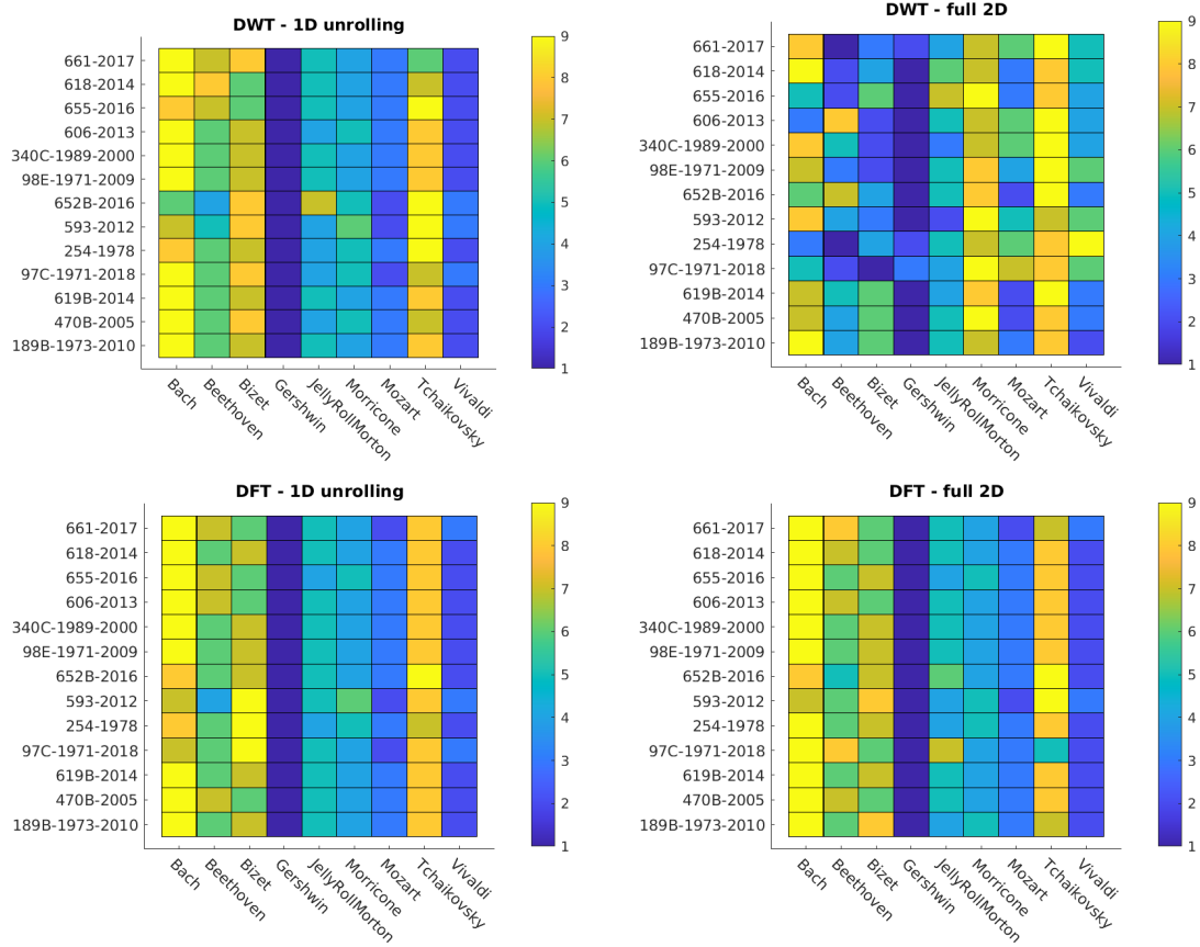
Figure 7: Similarity matrices between Morandini's paintings and composers' music, the dark blue colour corresponds to a greater similarity, the yellow to a lesser similarity. The top-right picture (DWT with full 2D transform) has been obtained by adopting the strategy of replicating the coefficients of the image's transform
