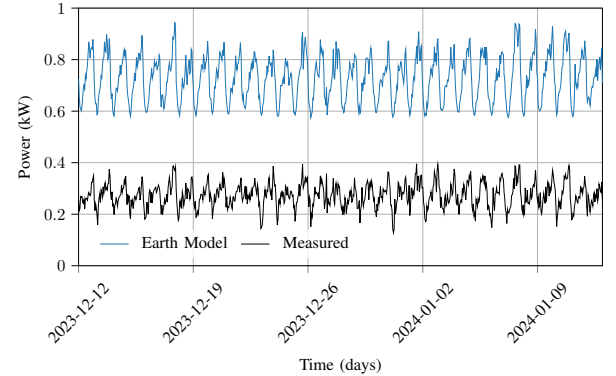
Fig. 2: Measured power demand and power demand computed by the EARTH model (in kW) for an LTE BS transmitting at 2100 MHz.
