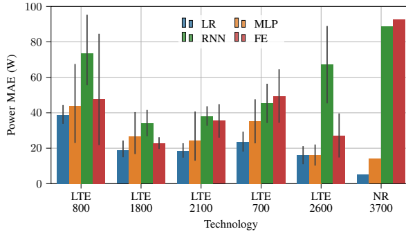
(a) MAE
