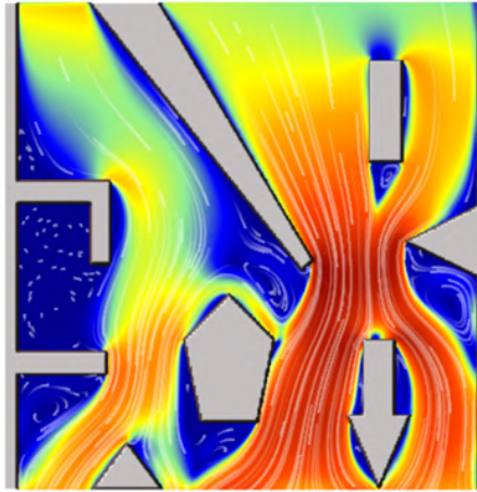
Figure 4.13: Computed streamlines of the flow field for the bathymetry in the right panel of Figure 4.10b. Flow from north to south.
