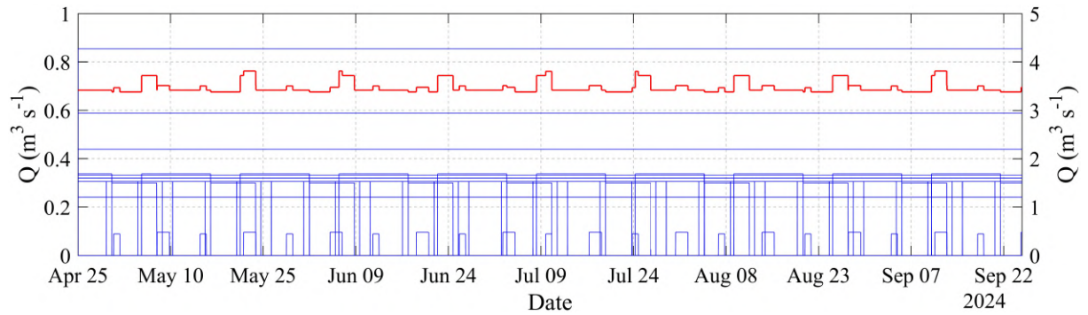
Figure 6.11: Timetable of the water shifts for the Diramatore Bruno Loffi Canal. The solid red line represents the sum of the delivered discharge along the channel.
