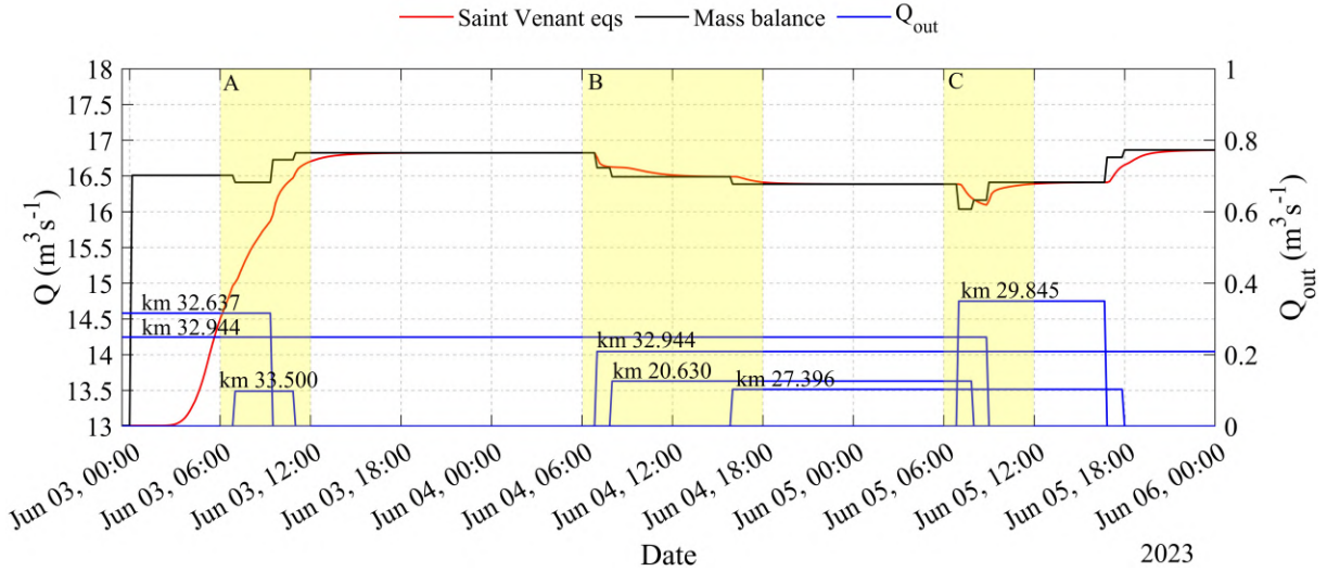
Figure 6.26: Comparison of the discharge variation over time obtained using the Saint-Venant Equations and the mass balance approach at the end of the domain (Tombe Morte) in the period from from June 3 to June 6. Note that two water whithdrwals points are placed at same transect km 32.944 because the gates are placed on the secondary channel Geronda Canal.
