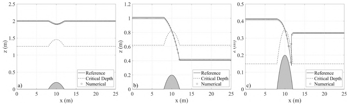
Figure 1.20: Comparison between analytical solutions e numerical solutions for flow over a bump a) subcritical flow, b) transcritical flow without shock, c) transcritical flow with shock.
