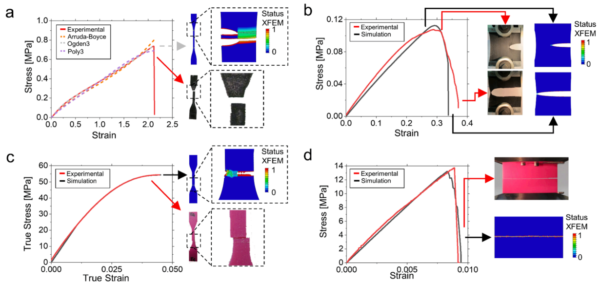
Fig. 3. (a) Comparison between the experimental and XFEM results for the (a, c) uniaxial tensile and (b, d) fracture test of (a, b) TangoBlackPlus and (c, d) Ver-o-Magenta. Status XFEM states the local crack propagation: being a full propagation the total element fracture is represented in red (Status XFEM = 1) and blue the opposite (Status XFEM = 0) [50]. (For interpretation of the references to colour in this figure legend, the reader is referred to the web version of this article.)
