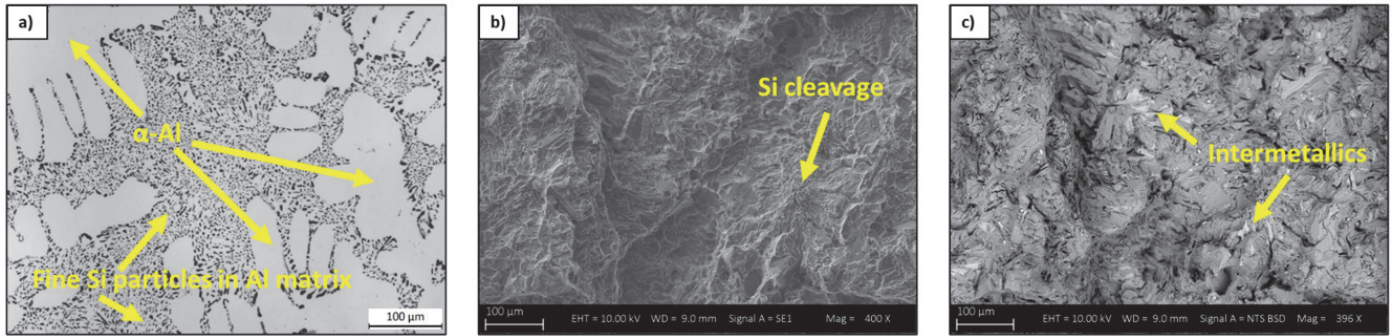
Figure 10: HIP 50 +T6 treated specimen: (a) microstructure at high magnification by optical microscopy; (b-c) fracture surface by scanning electron microscopy.
