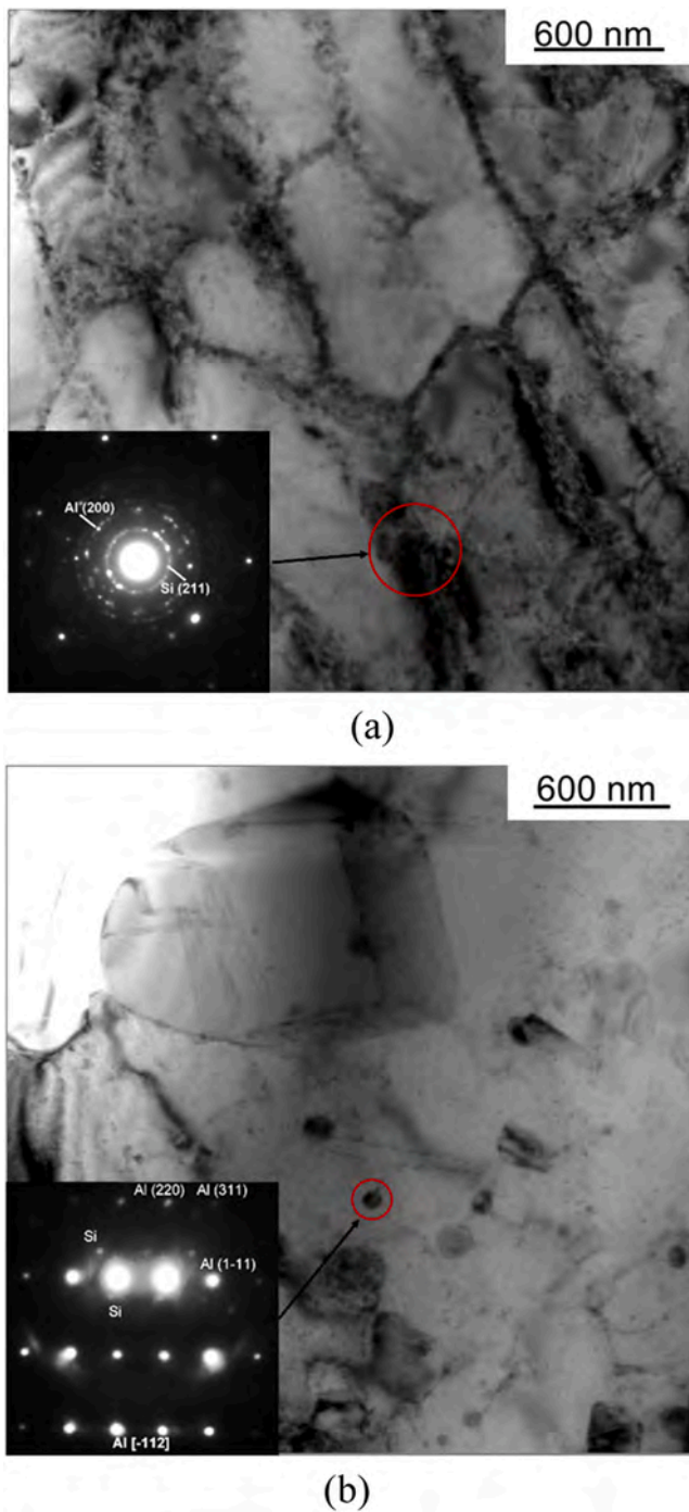
Fig. 6. Additive manufactured (AM) alloy: TEM micrograph in (a) shows elongated cells of \sim 400 nm while rounded and irregular shaped precipitates of very small size (100–150 nm) can be observed in (b). Insets in (a) and (b) show SAEDPs taken from the rounded red area of the micrographs. Both SAEDPs reveal the presence of Si particles. In (b) the Al-matrix zone axis is Al [-112] , [-112] .
