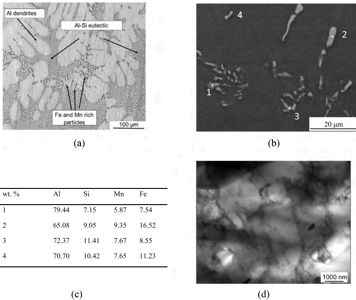
Fig. 1. As-cast (AC) alloy: LM micrograph in (a) shows the Al dendritic structure surrounded by a fine Al-Si eutectic and particles with elongated shape. The Chinese script morphology of these particles is displayed at higher magnification in the SEM image in (b). Some of them, indicated in (b), have been analyzed by EDS and the compositions are reported in (c). TEM micrograph in (d) displays the cell structure formed by dislocations in the Al matrix.
