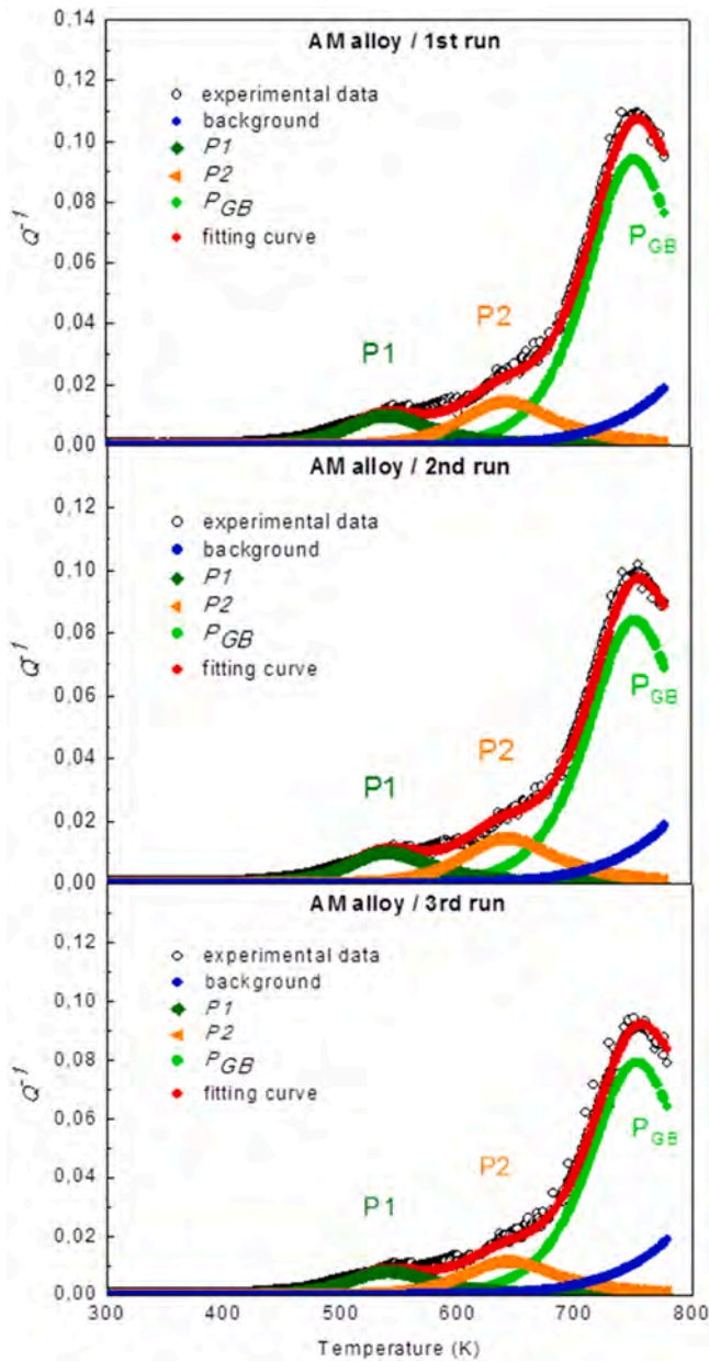
Fig. 8. Additive manufactured (AM) alloy: the Q^{-1} curves vs. temperature recorded in 1st, 2nd and 3rd runs (open circles) have been fitted by the sum of four contributions, namely the background (blue points), the peaks P1 (olive points), P2 (orange points) and P_{GB} (green points). The fitting curve is indicated by red points. The resonance frequency is 670 Hz.
