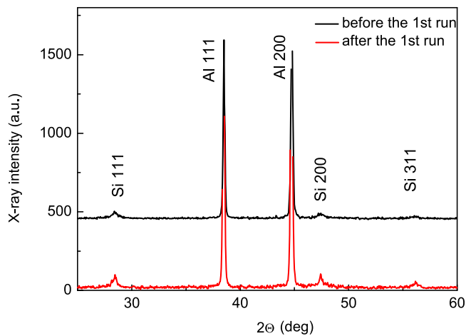
Fig. 11. XRD patterns of the additive manufactured (AM) alloy before and after the 1st test run.
