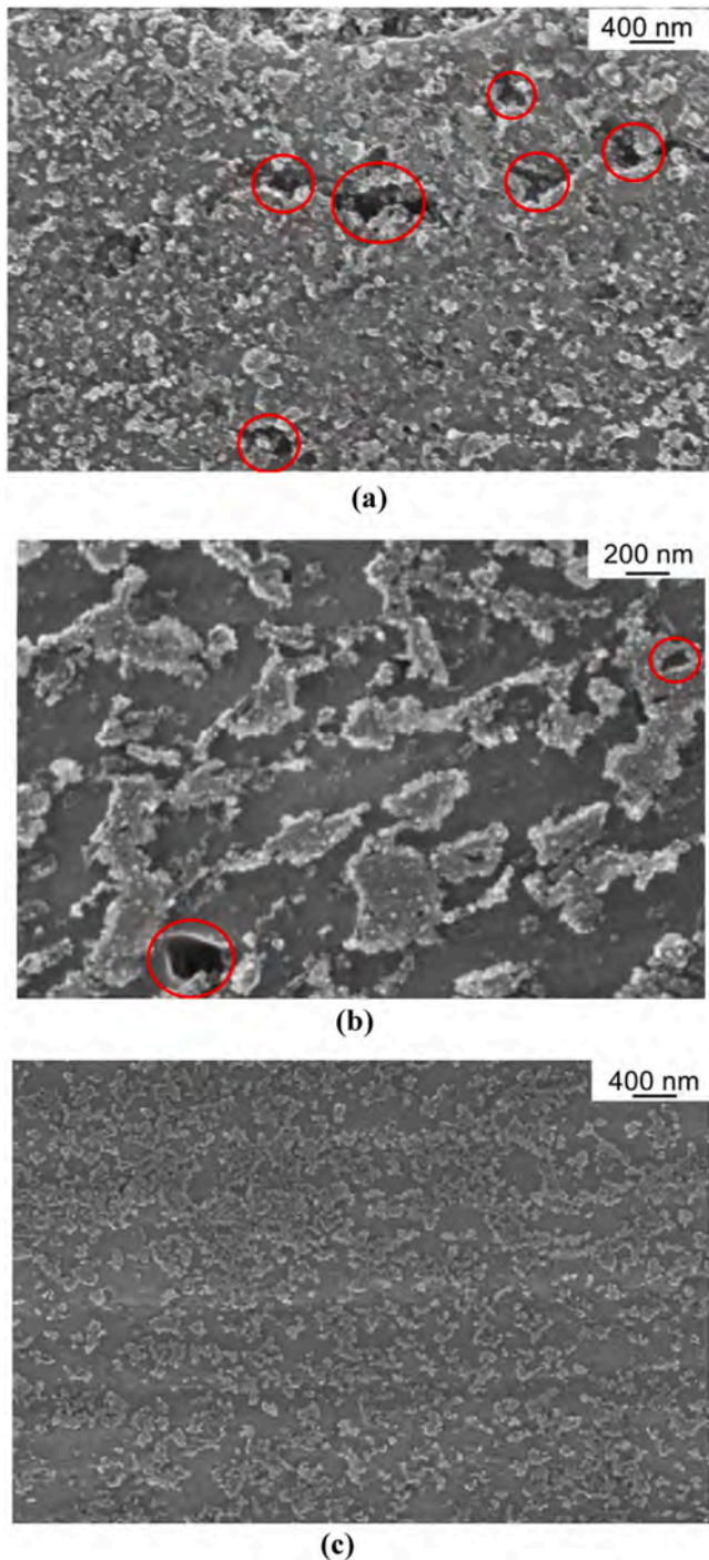
Fig. 13. FEG-SEM micrographs of as-built additive manufactured (AM) alloy at increasing magnification (a and b) and after an MS test run with heating up to 485 K (c). Pores are indicated by red circles in (a) and (b).
