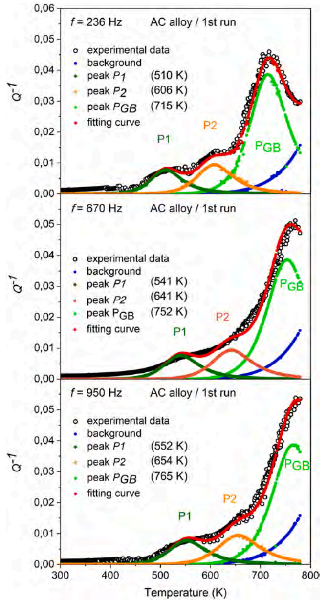
Fig. 3. As-cast (AC) alloy: the Q^{-1} curves vs. temperature (open circles) recorded with different resonance frequencies (236, 670 and 950 Hz) have been fitted by the sum of four contributions, namely the background (blue points), the peaks P1 (olive points), P2 (orange points) and P_{GB} (green points). The fitting curve is indicated by red points. The central positions of P1 , P2 and P_{GB} peaks, reported in each graph, change with the frequency.
