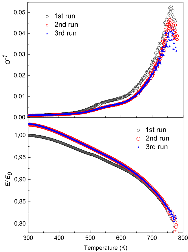
Fig. 2. As-cast (AC) alloy: Q^{-1} and dynamic modulus E vs. temperature measured in three successive test runs. Dynamic modulus values are normalized to the initial value E_0 (at room temperature, before the 1st run). The initial resonance frequency at room temperature is 670 Hz.
