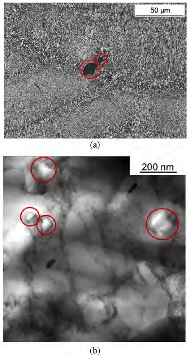
Fig. 7. Additive manufactured (AM) alloy: pores of great (SEM micrograph in a) and small size (TEM micrograph in b) are evidenced by red circles.
