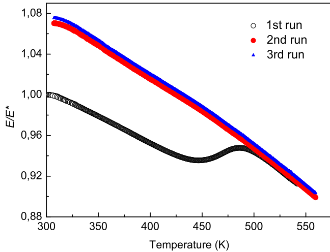
Fig. 10. Dynamic modulus E vs. temperature of an additive manufactured (AM) sample measured in three successive test runs. The values of dynamic modulus are normalized to the value E^* measured at room temperature in the 1st test run.
