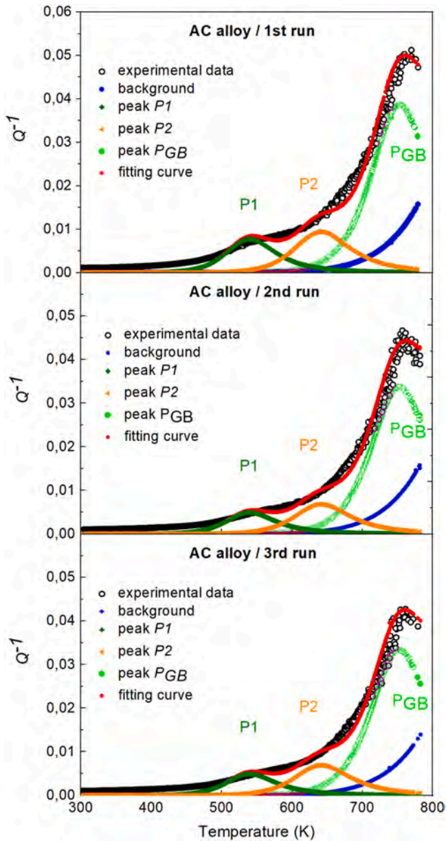
Fig. 4. As-cast (AC) alloy: the Q^{-1} curves vs. temperature recorded in 1st, 2nd and 3rd runs (open circles) have been fitted by the sum of four contributions, namely the background (blue points), the peaks P1 (olive points), P2 (orange points) and P_{GB} (green points). The fitting curve is indicated by red points. The resonance frequency is 670 Hz.
