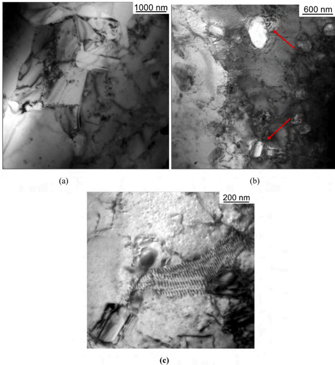
Fig. 12. TEM images of additive manufactured (AM) alloy after the 1st test run. Elongated cells have been replaced by equiaxed cells of larger size (a). Pores of large size are indicated by red arrows (b). In (c) an array of kinked dislocations is observed.
