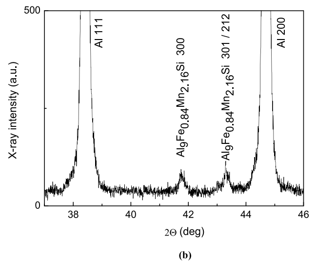
Fig. 9. XRD patterns of as-cast (AC) and additive manufactured (AM) alloys (a) recorded with 2\theta steps of 0.05^\circ and counting time per step of 2 s. Figure (b) displays a part of the XRD pattern of as-cast (AC) alloy recorded with higher resolution ( 2\theta steps of 0.005^\circ ) and longer counting time (20 s) to evidence two weak peaks which result to correspond to the Al_9Fe_{0.84}Mn_{2.16}Si compound.
