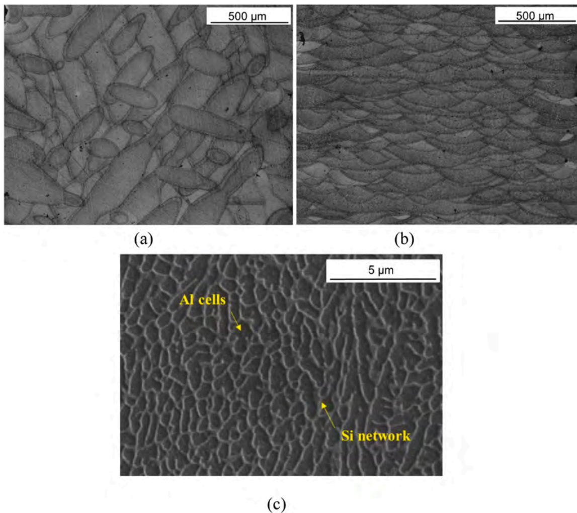
Fig. 5. Additive manufactured (AM) alloy: LM micrographs of horizontal and vertical sections are shown in (a) and (b), respectively. The SEM image at higher magnification in (c) shows the Al cellular structure surrounded by a network of Si particles.
